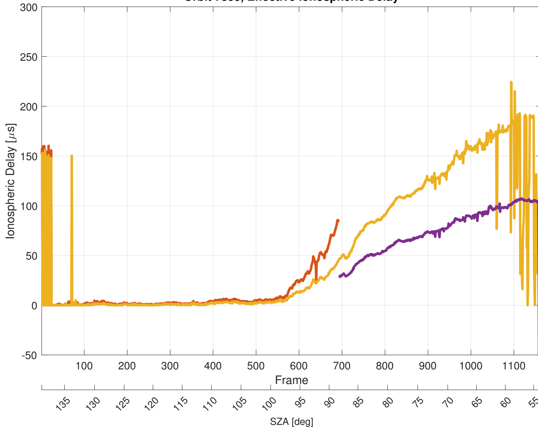
Orbit 7883, Effective Ionospheric Delay
