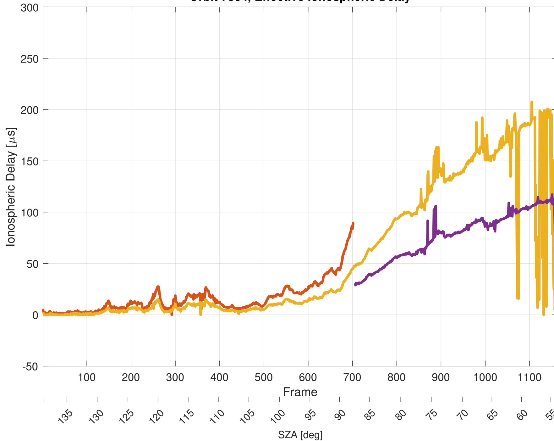
Orbit 7884, Effective Ionospheric Delay
