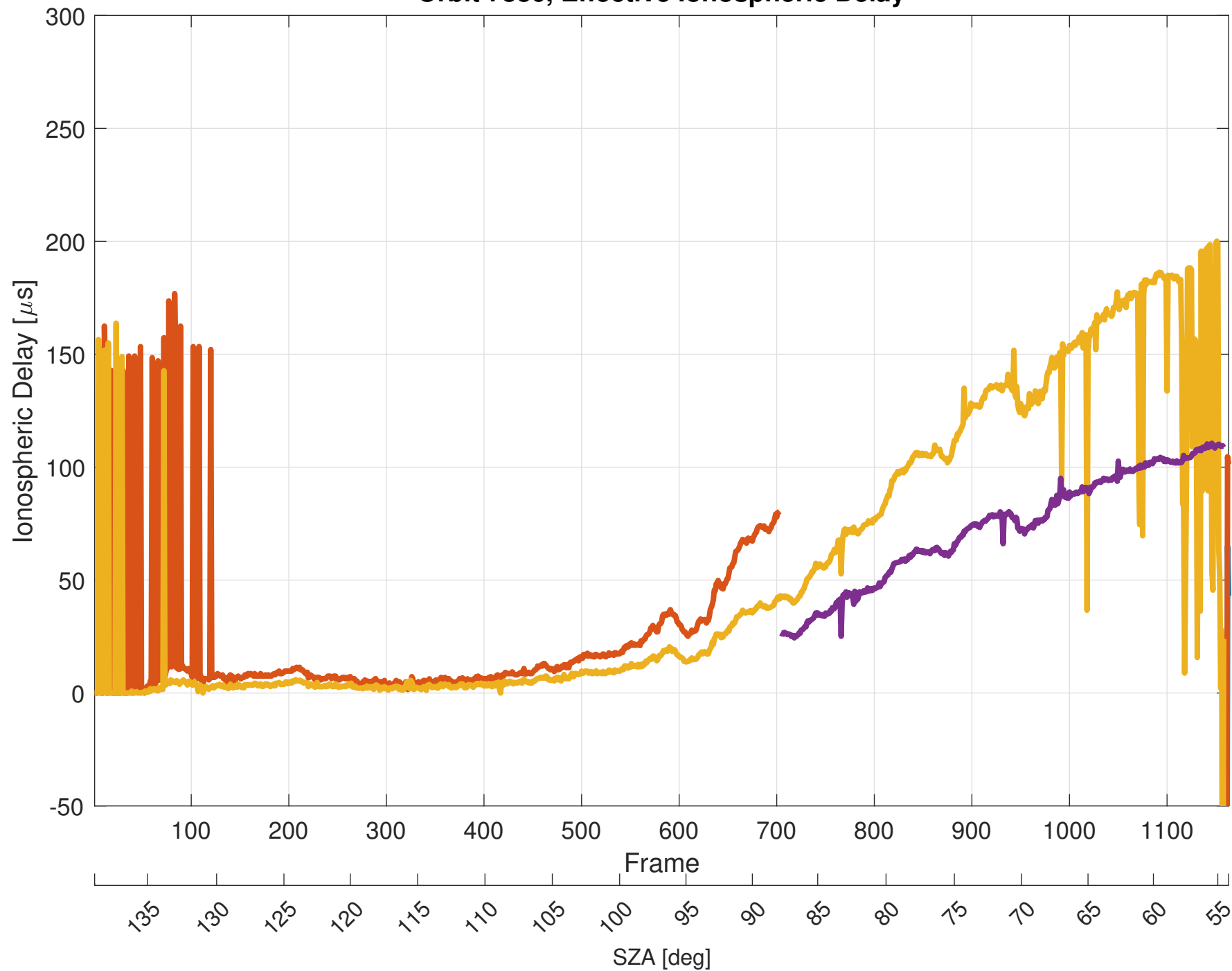
Orbit 7886, Effective Ionospheric Delay
