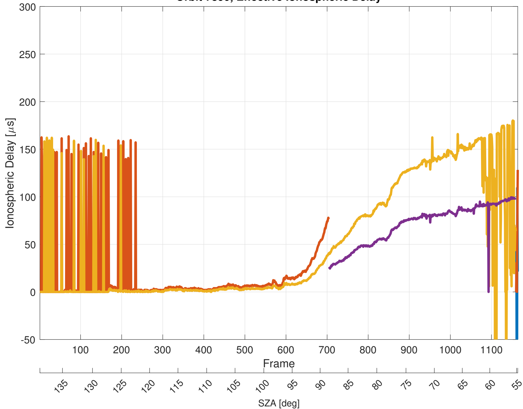
Orbit 7890, Effective Ionospheric Delay
