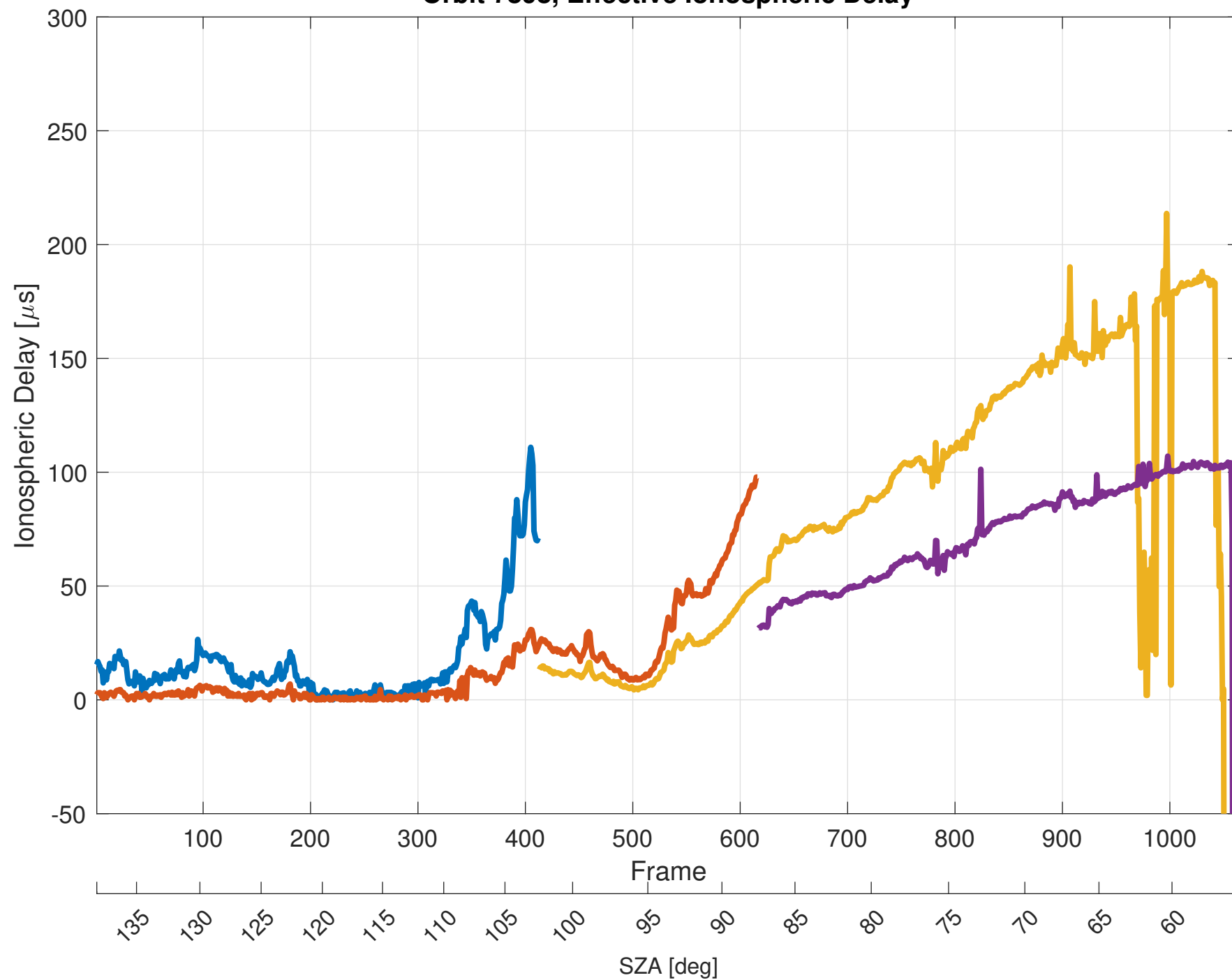
Orbit 7898, Effective Ionospheric Delay
