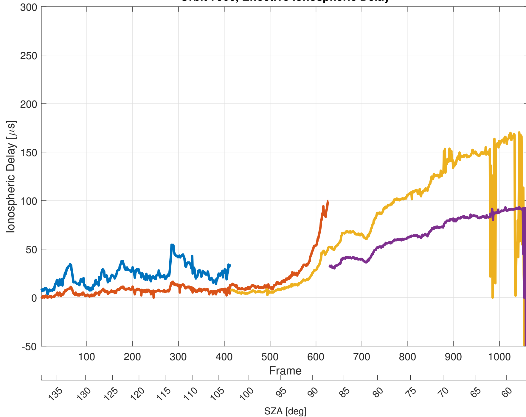
Orbit 7906, Effective Ionospheric Delay
