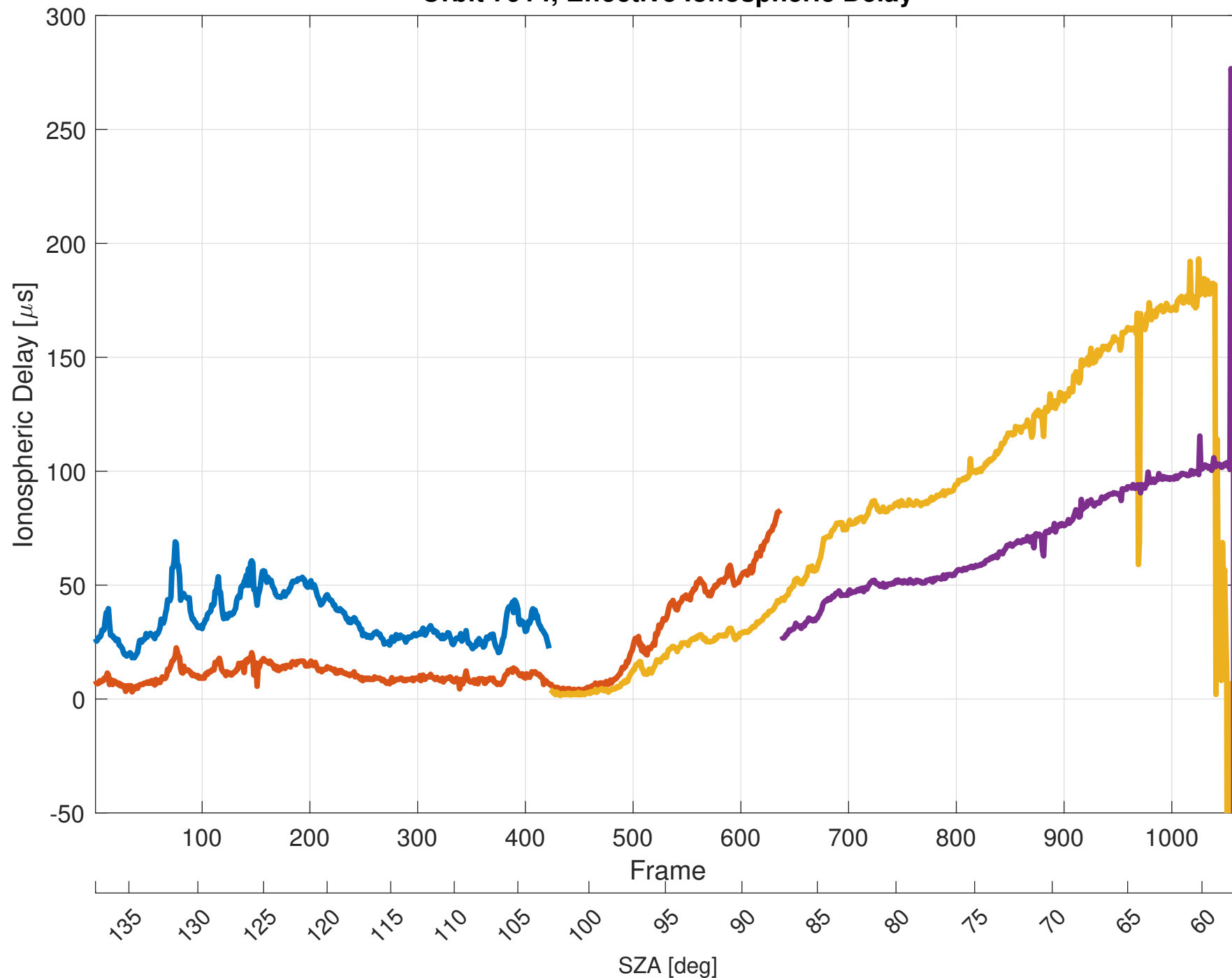
Orbit 7914, Effective Ionospheric Delay
