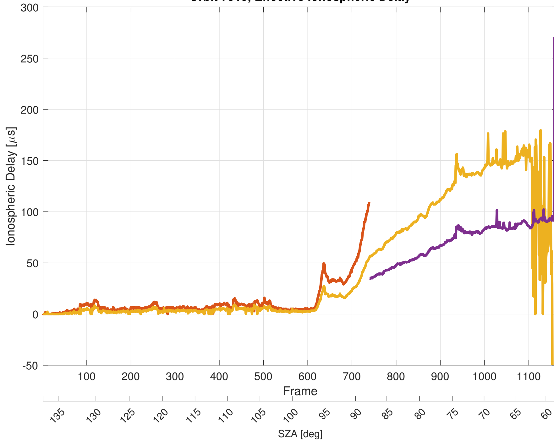
Orbit 7919, Effective Ionospheric Delay
