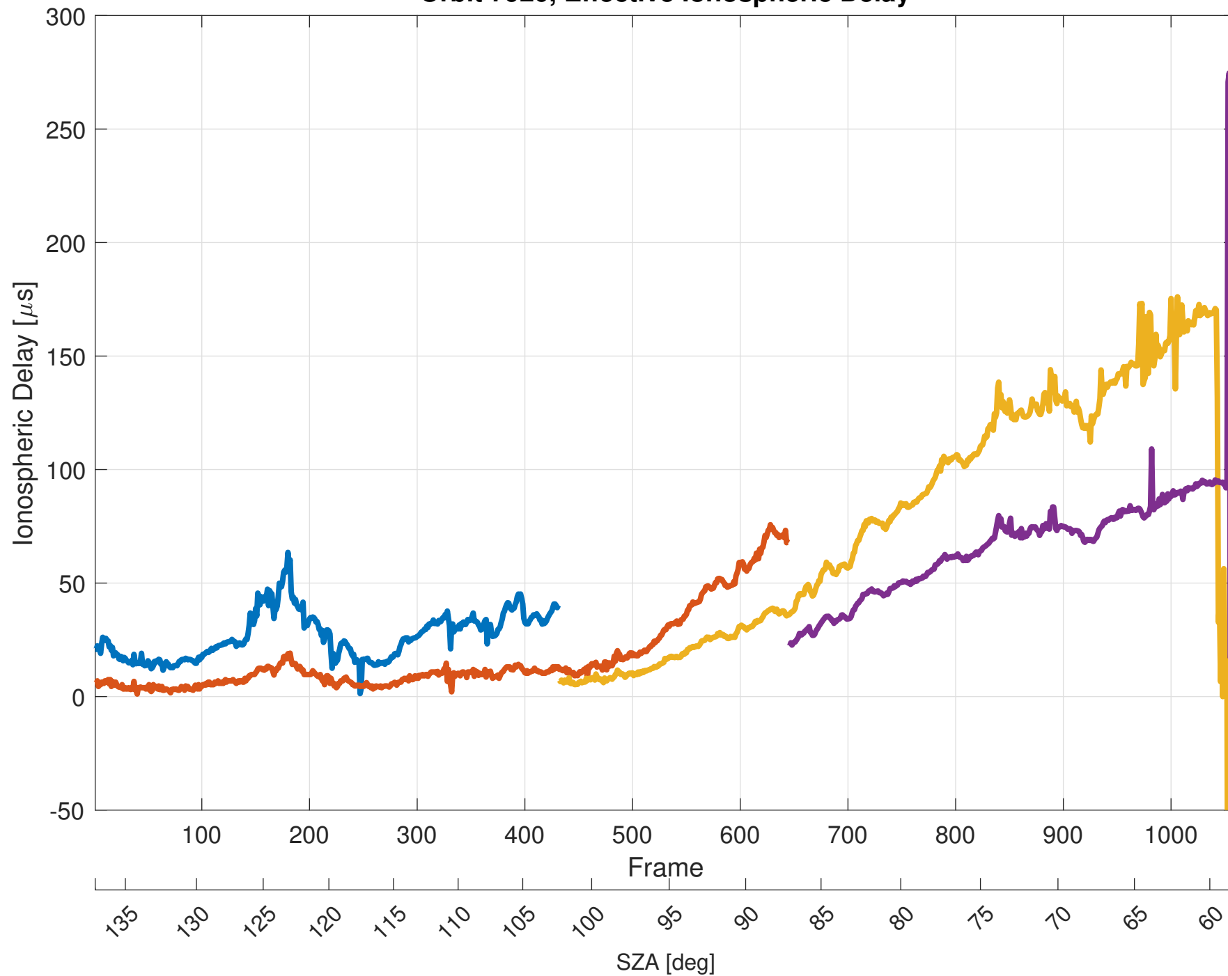
Orbit 7920, Effective Ionospheric Delay
