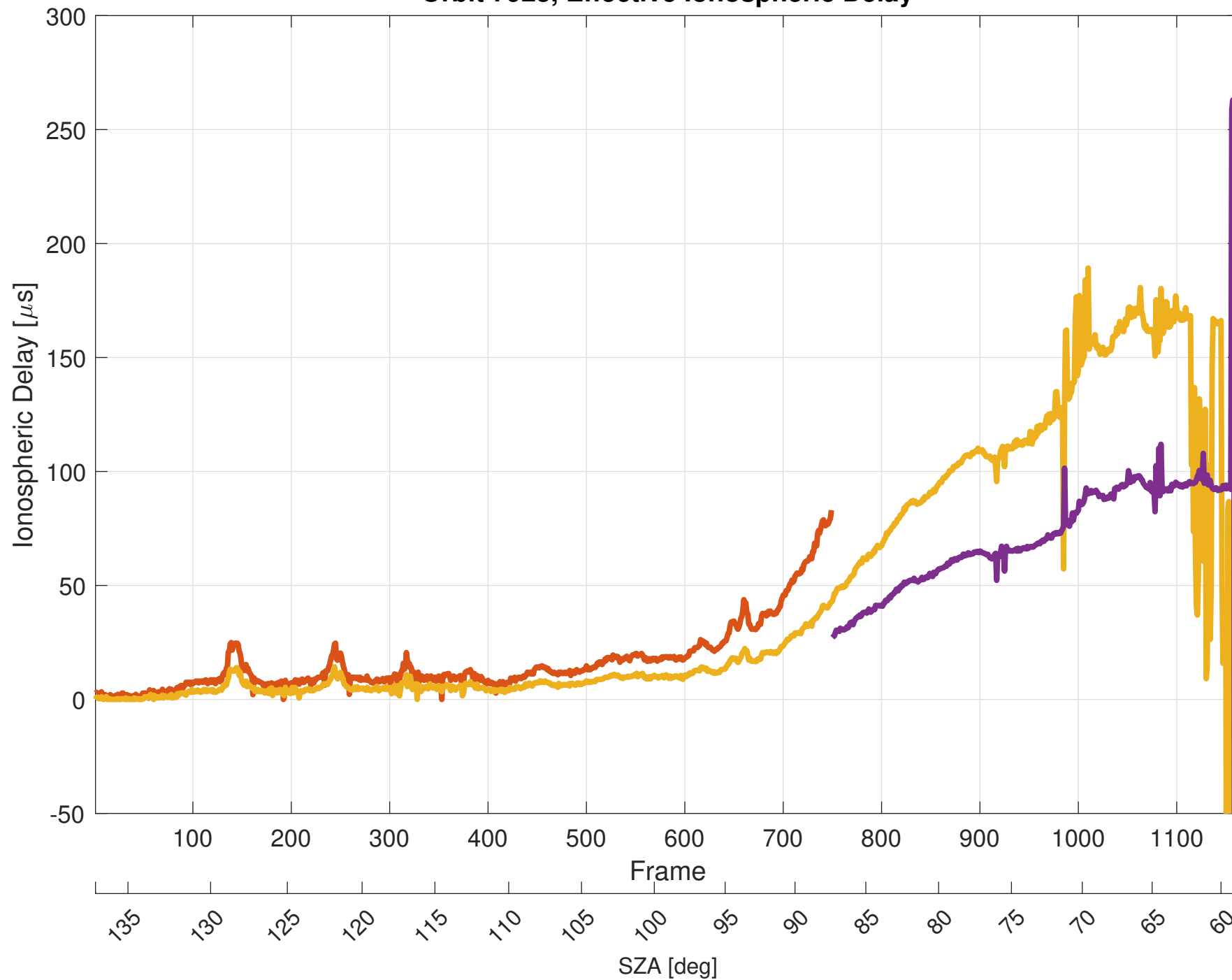
Orbit 7923, Effective Ionospheric Delay
