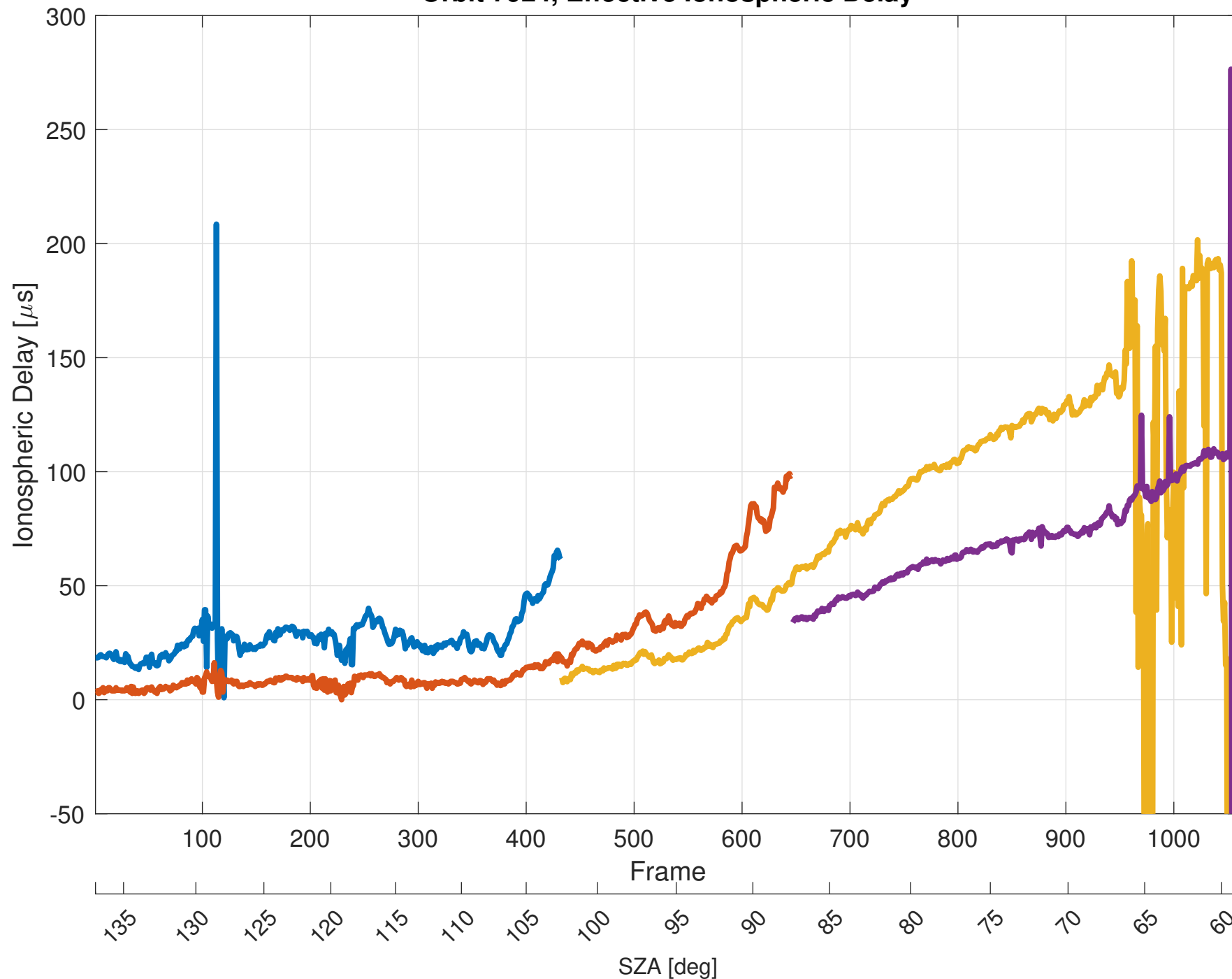
Orbit 7924, Effective Ionospheric Delay
