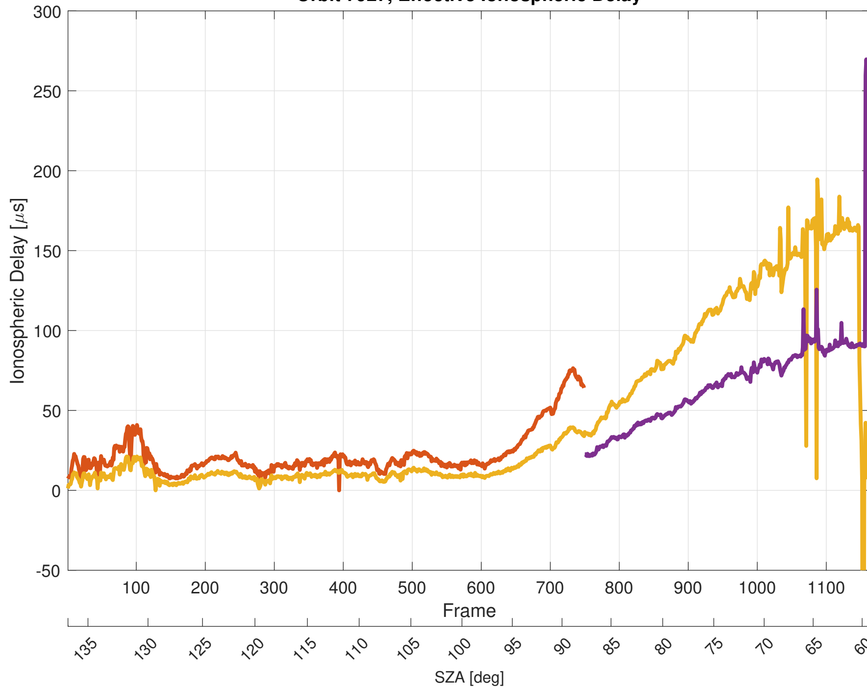
Orbit 7927, Effective Ionospheric Delay
