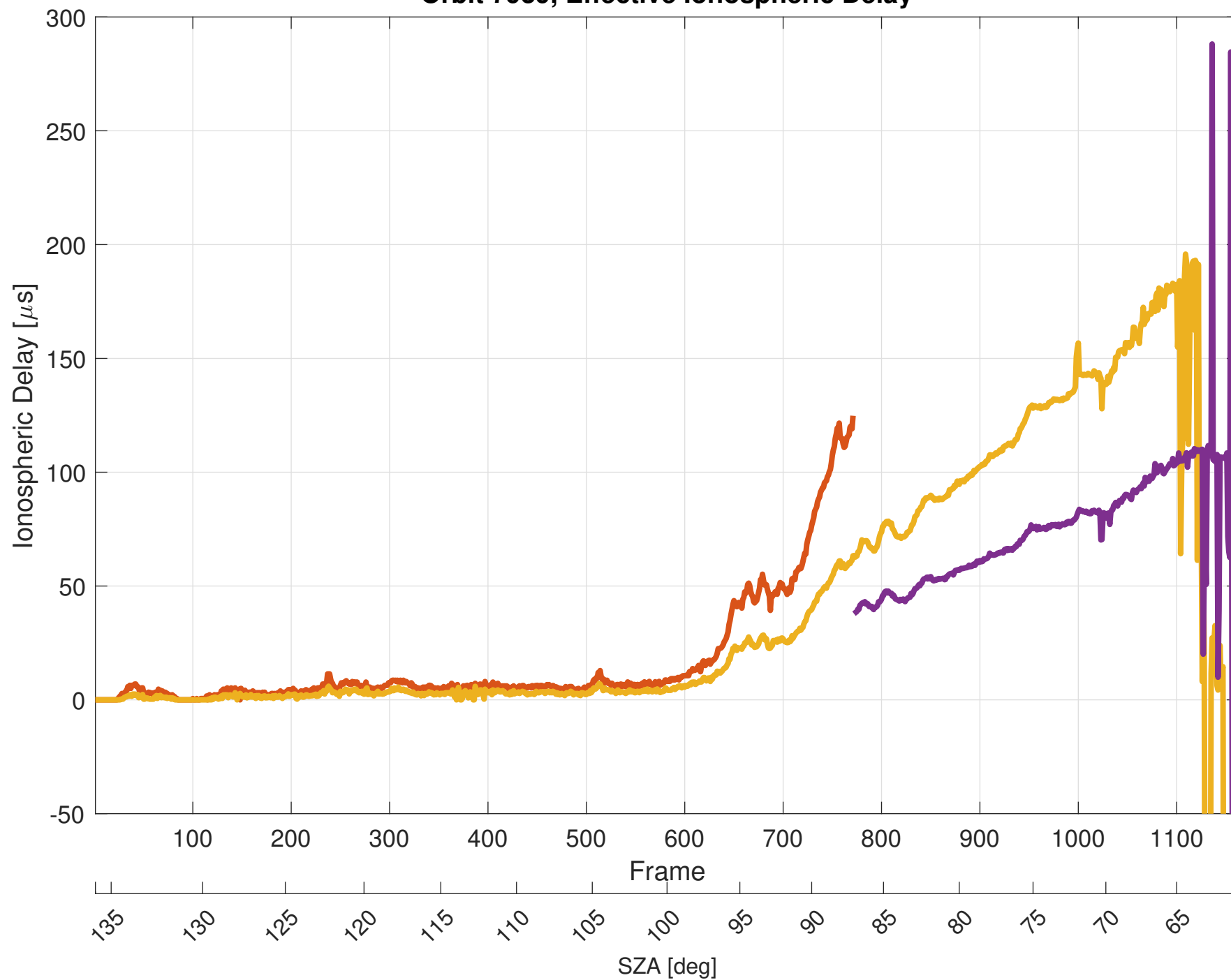
Orbit 7939, Effective Ionospheric Delay
