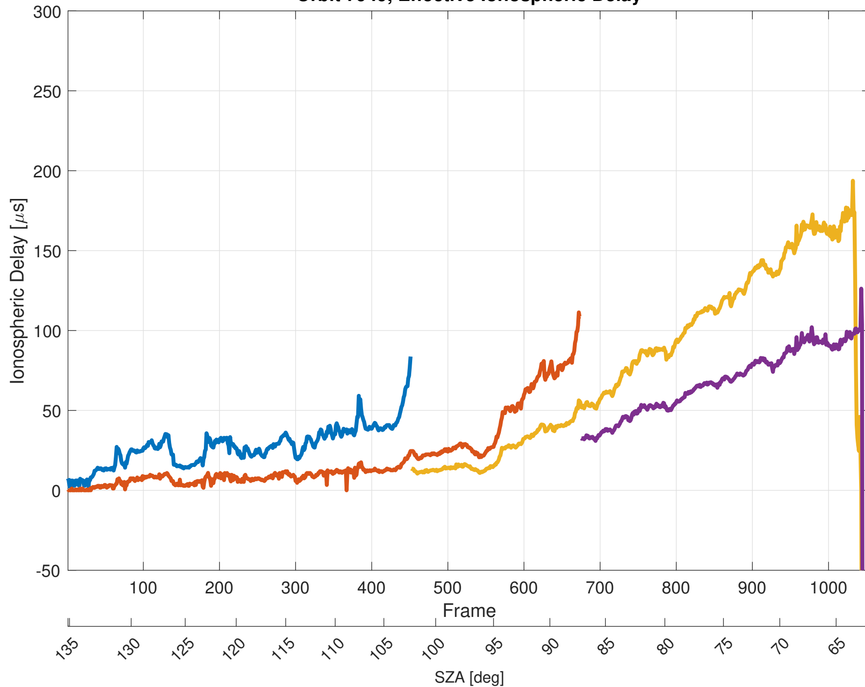
Orbit 7949, Effective Ionospheric Delay
