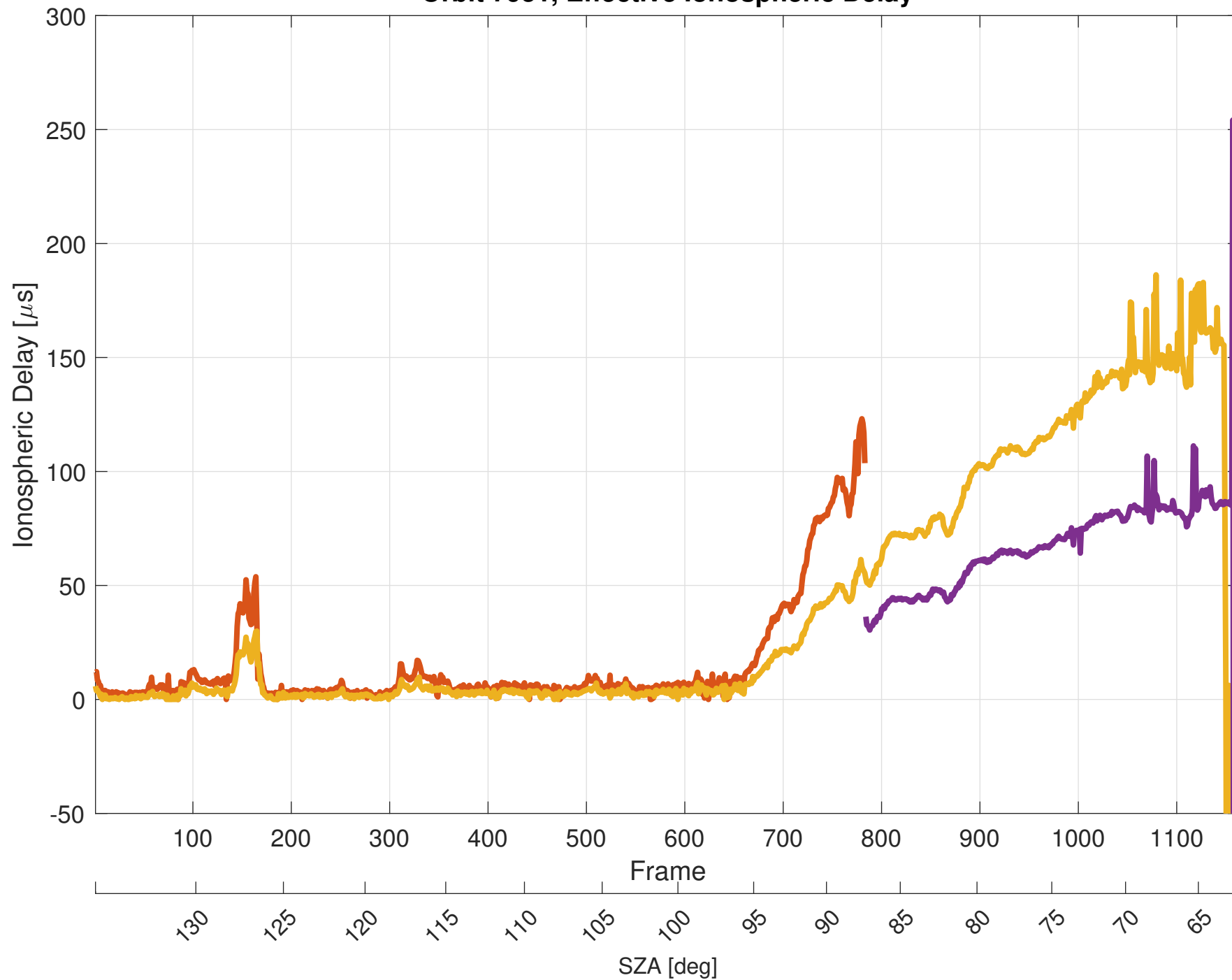
Orbit 7951, Effective Ionospheric Delay
