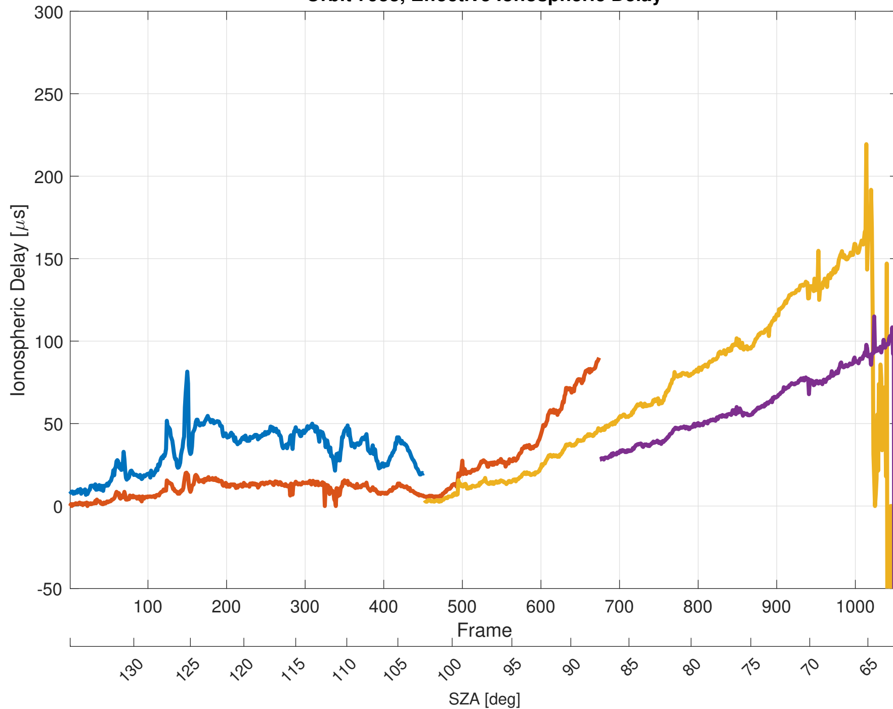
Orbit 7953, Effective Ionospheric Delay
