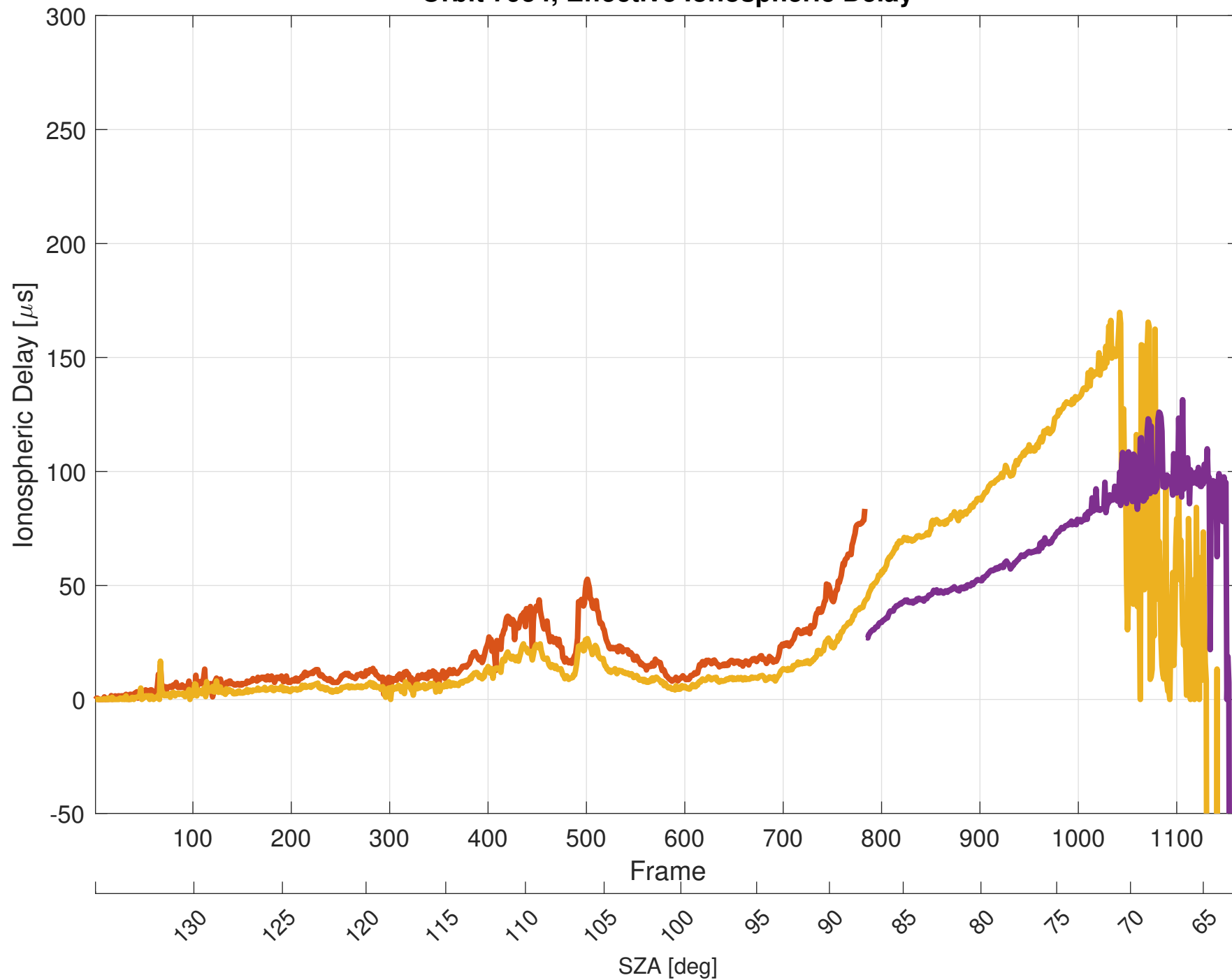
Orbit 7954, Effective Ionospheric Delay
