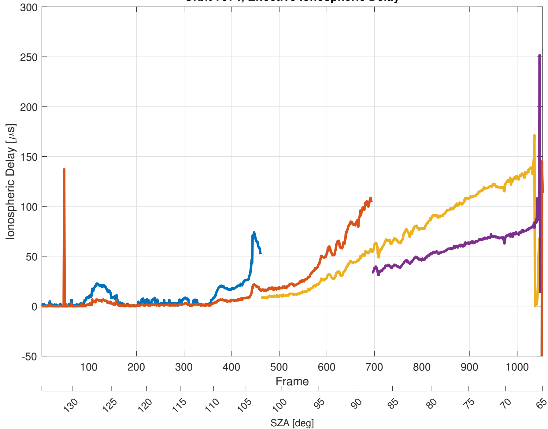
Orbit 7974, Effective Ionospheric Delay
