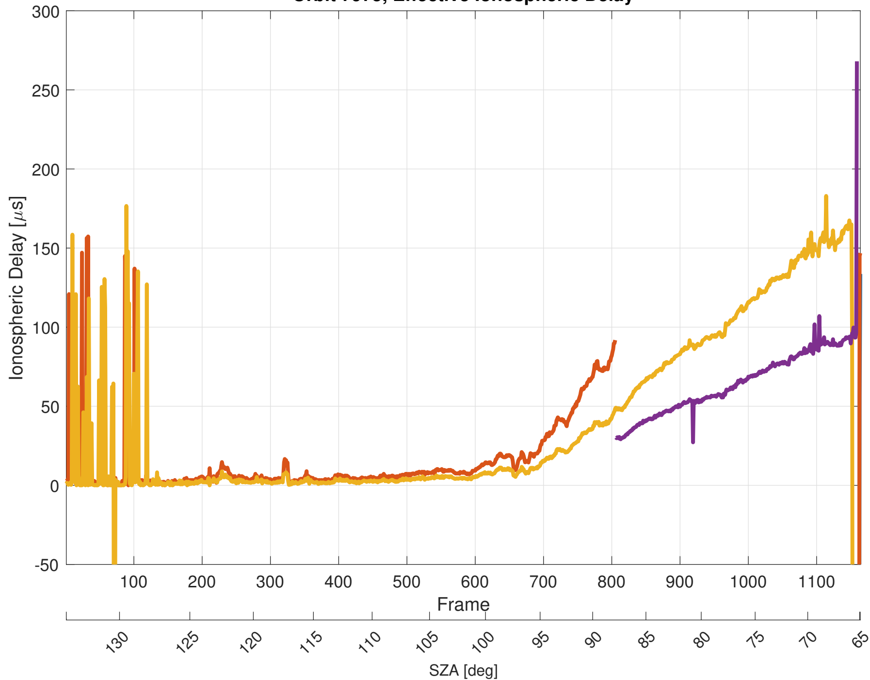
Orbit 7975, Effective Ionospheric Delay
