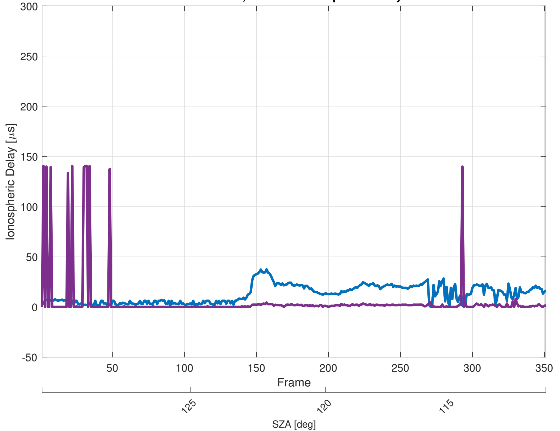
Orbit 8016, Effective Ionospheric Delay
