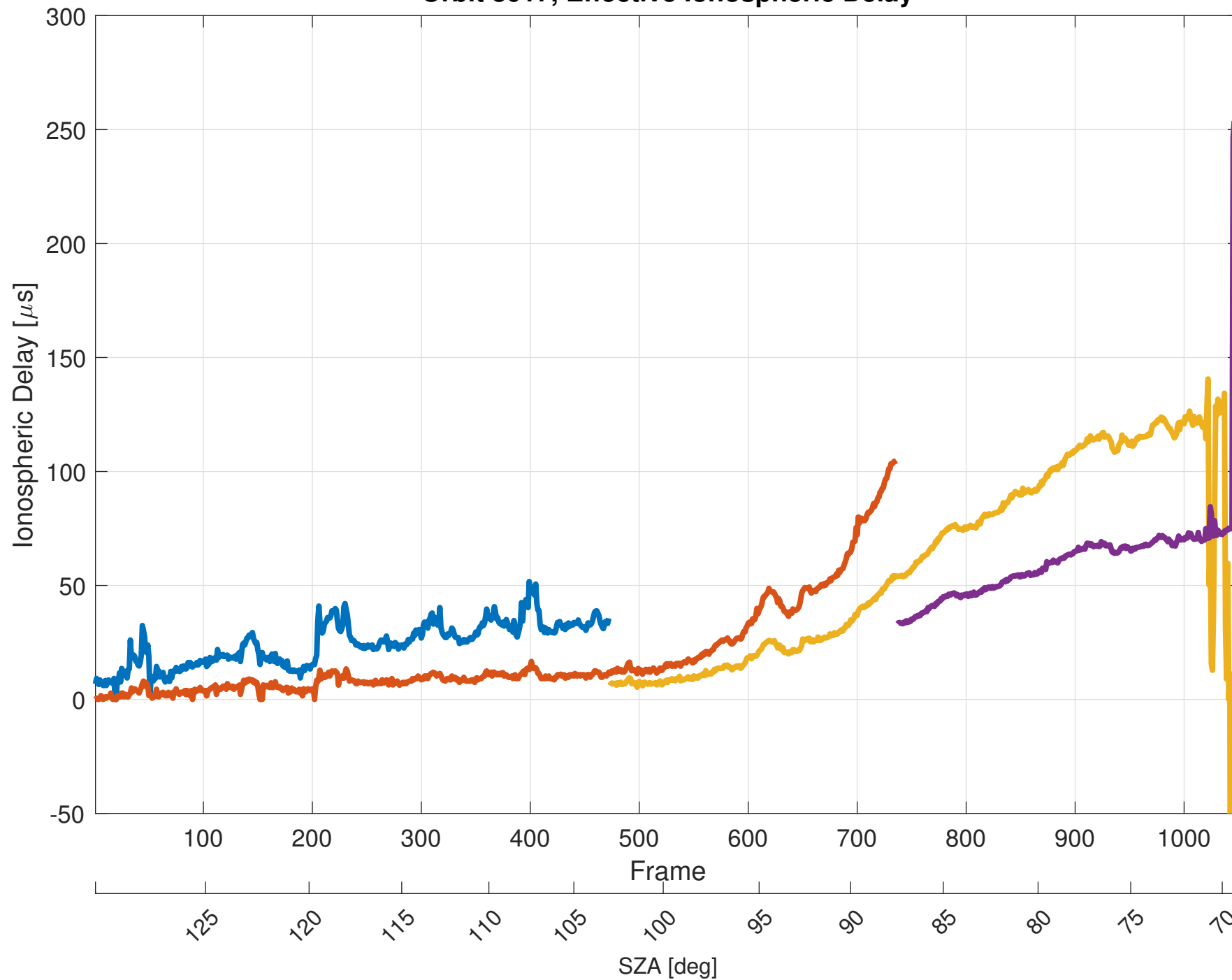
Orbit 8017, Effective Ionospheric Delay
