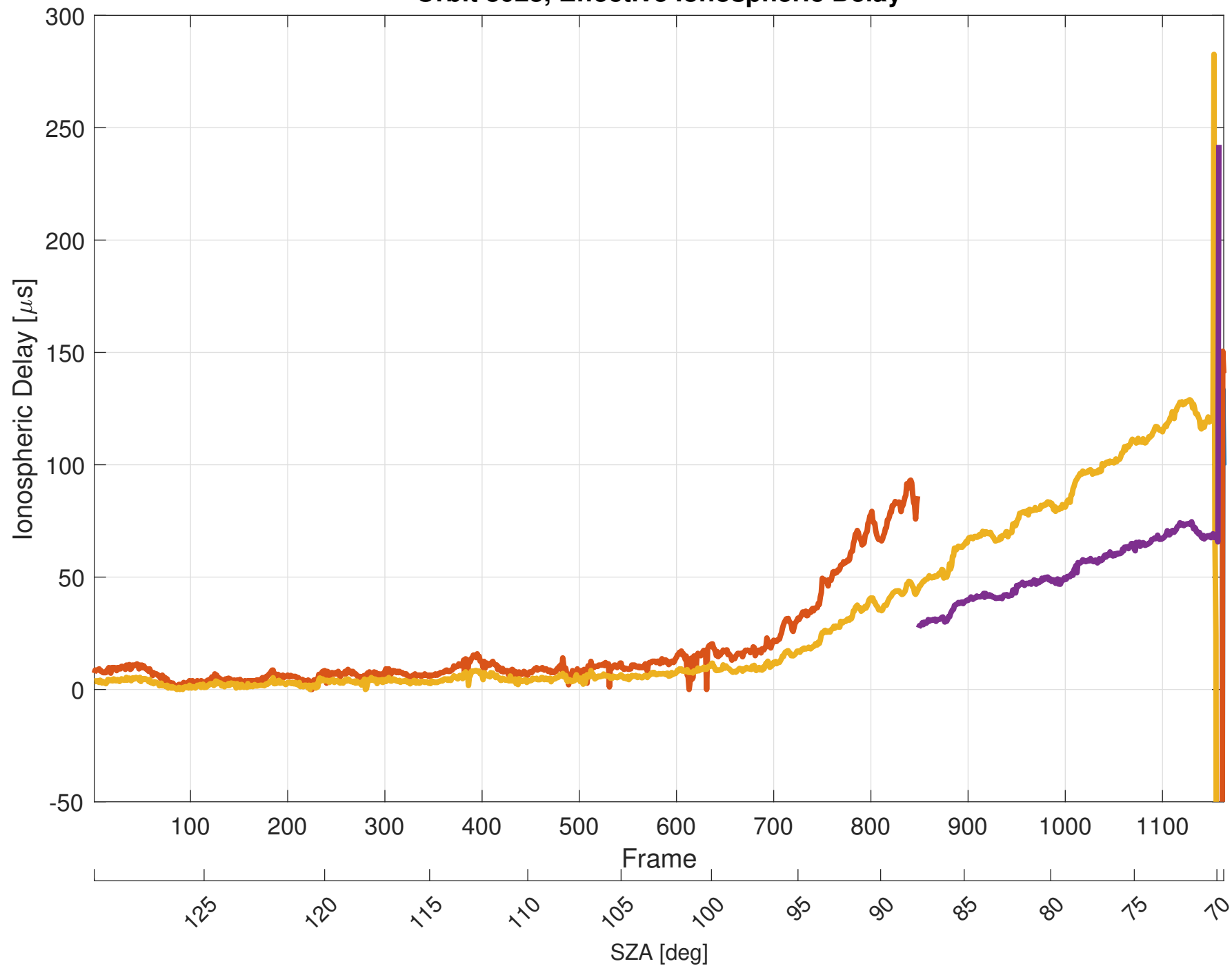
Orbit 8023, Effective Ionospheric Delay
