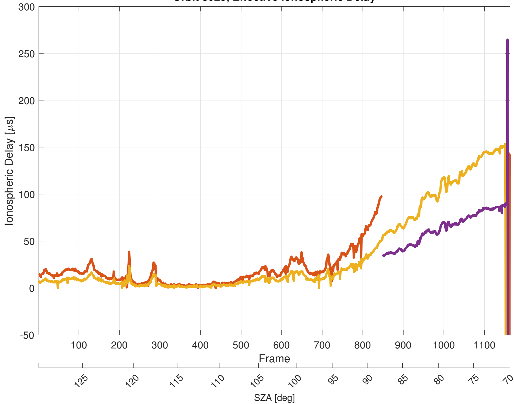
Orbit 8025, Effective Ionospheric Delay
