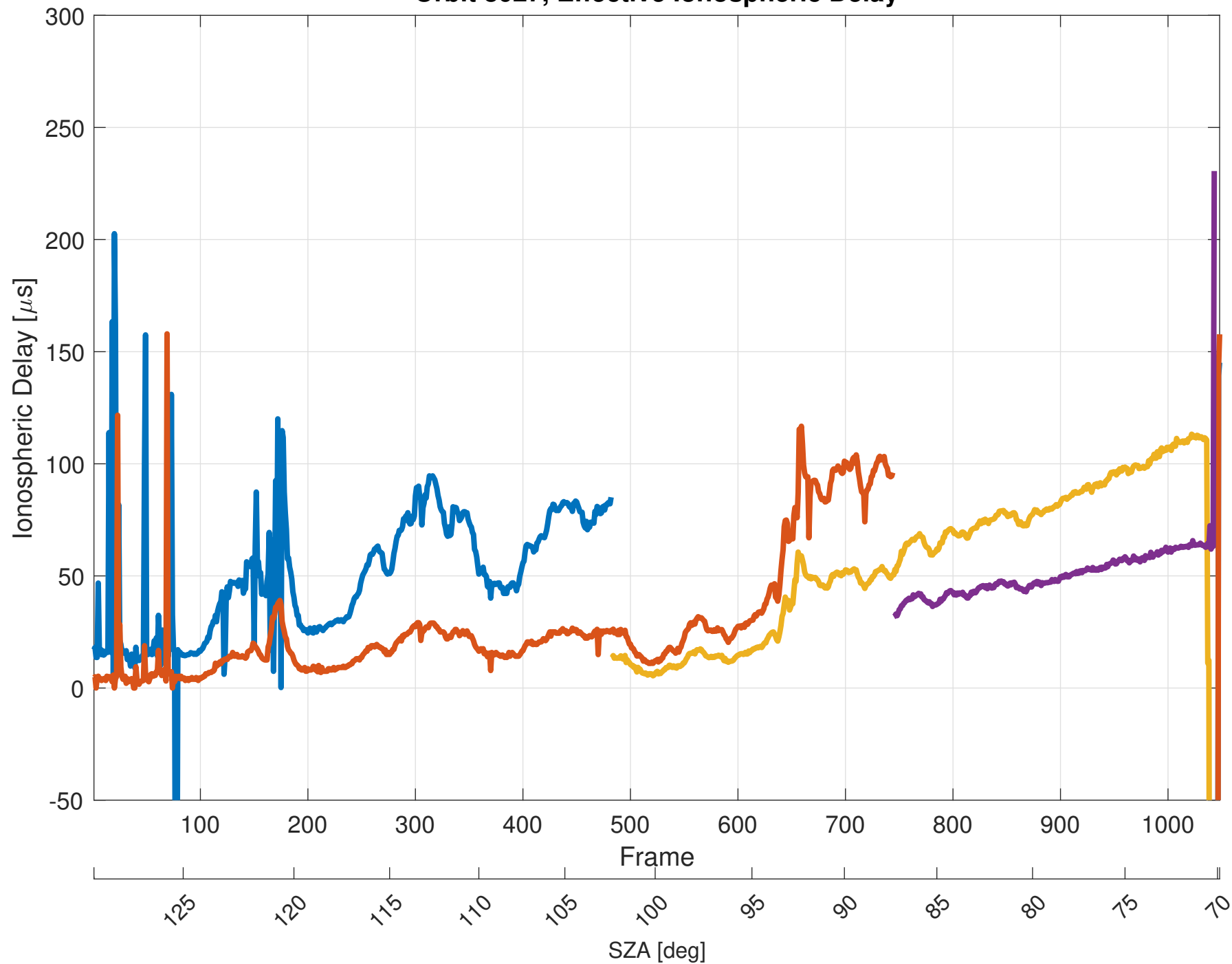
Orbit 8027, Effective Ionospheric Delay
