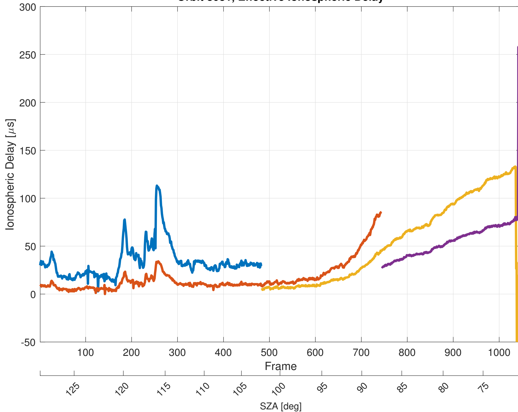
Orbit 8031, Effective Ionospheric Delay
