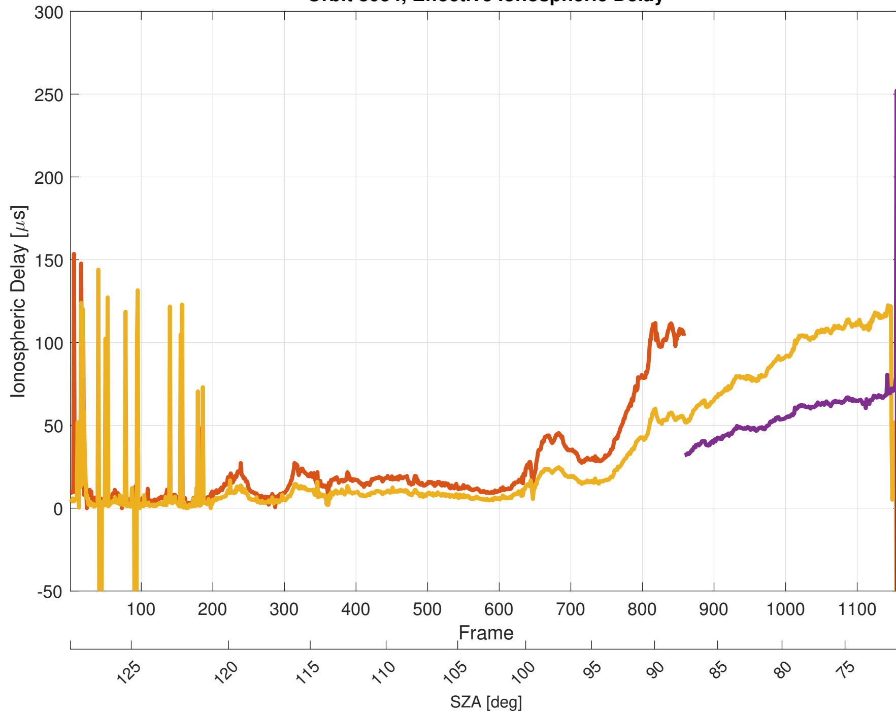
Orbit 8034, Effective Ionospheric Delay
