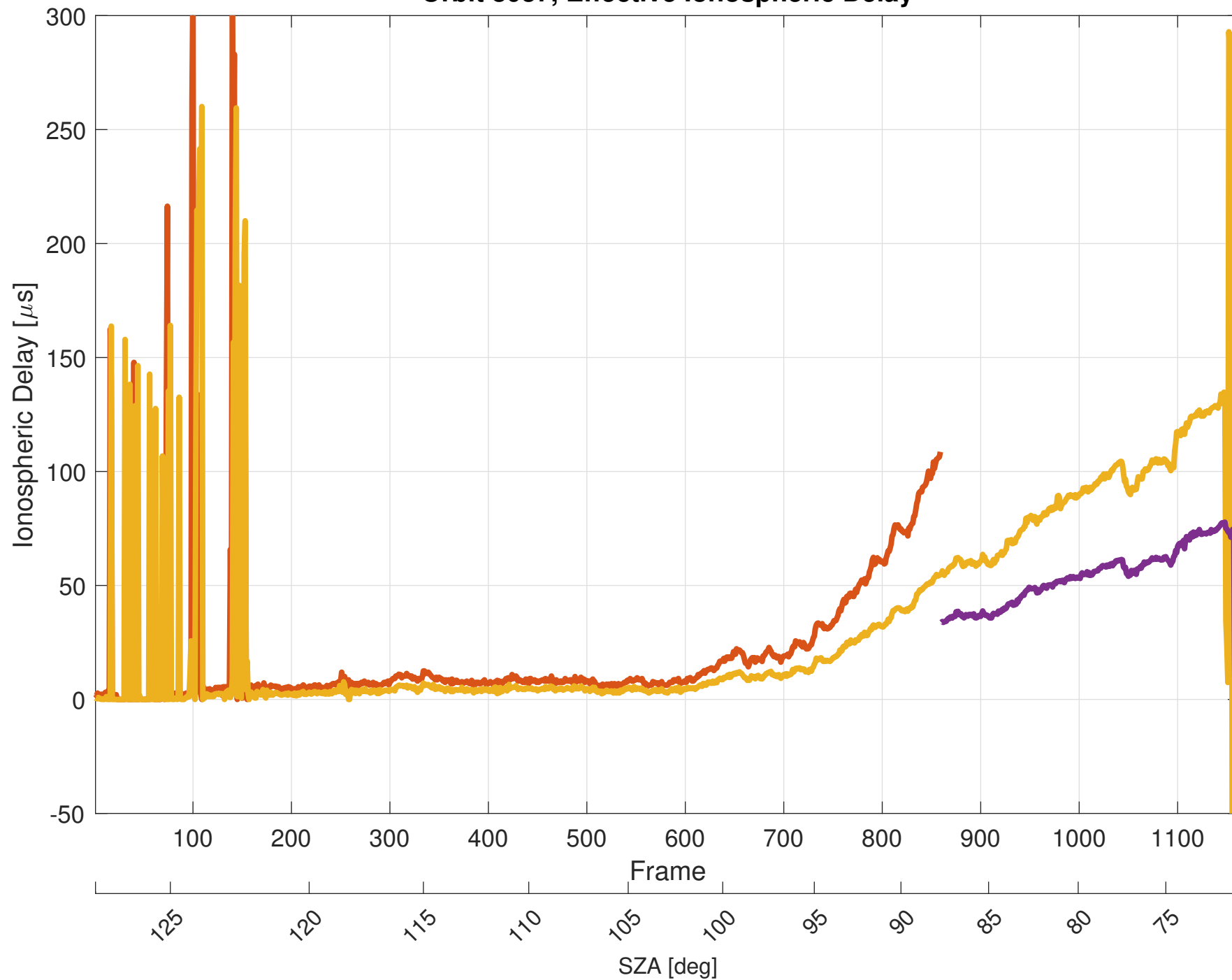
Orbit 8037, Effective Ionospheric Delay
