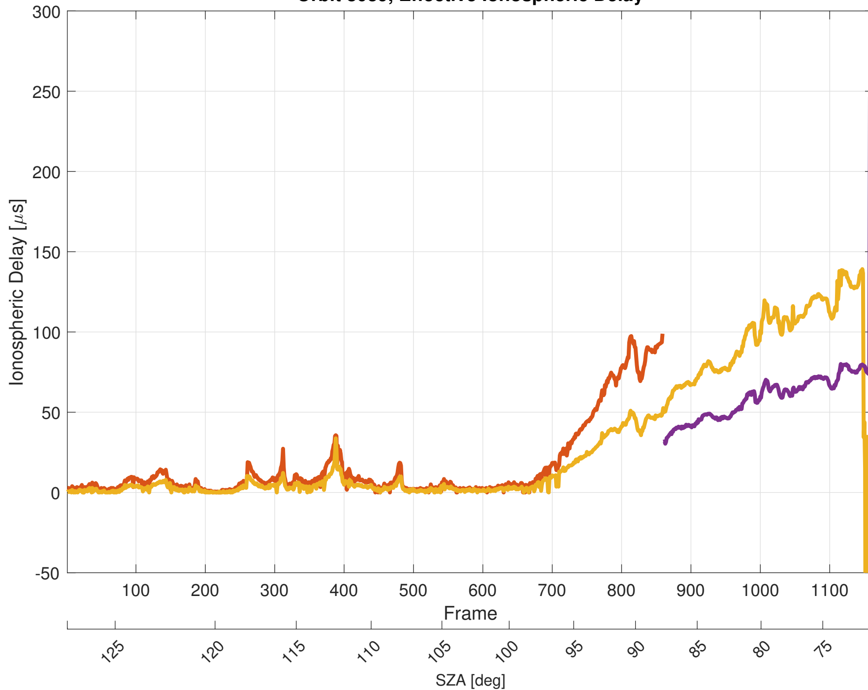
Orbit 8039, Effective Ionospheric Delay
