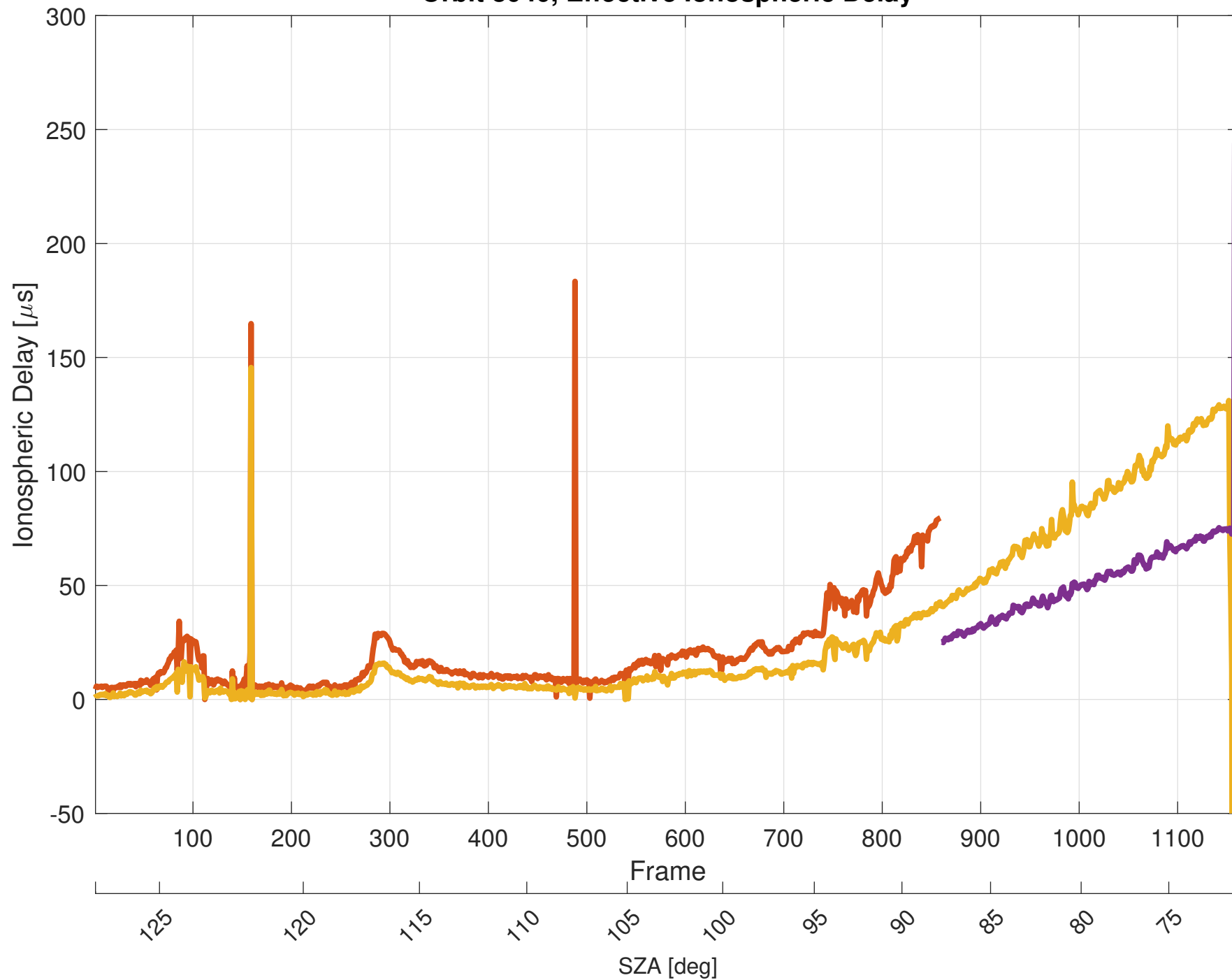
Orbit 8040, Effective Ionospheric Delay
