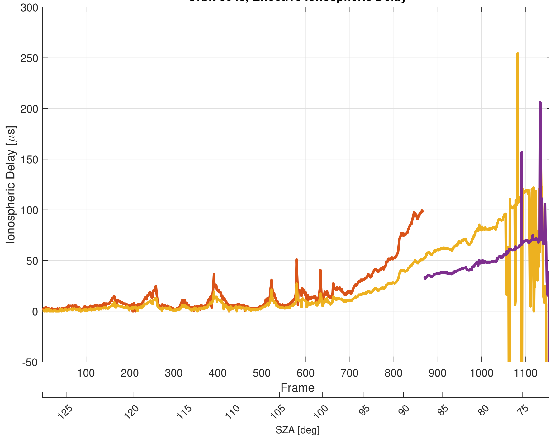
Orbit 8043, Effective Ionospheric Delay
