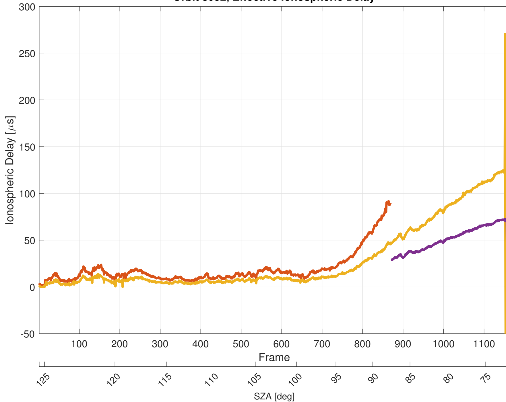
Orbit 8052, Effective Ionospheric Delay
