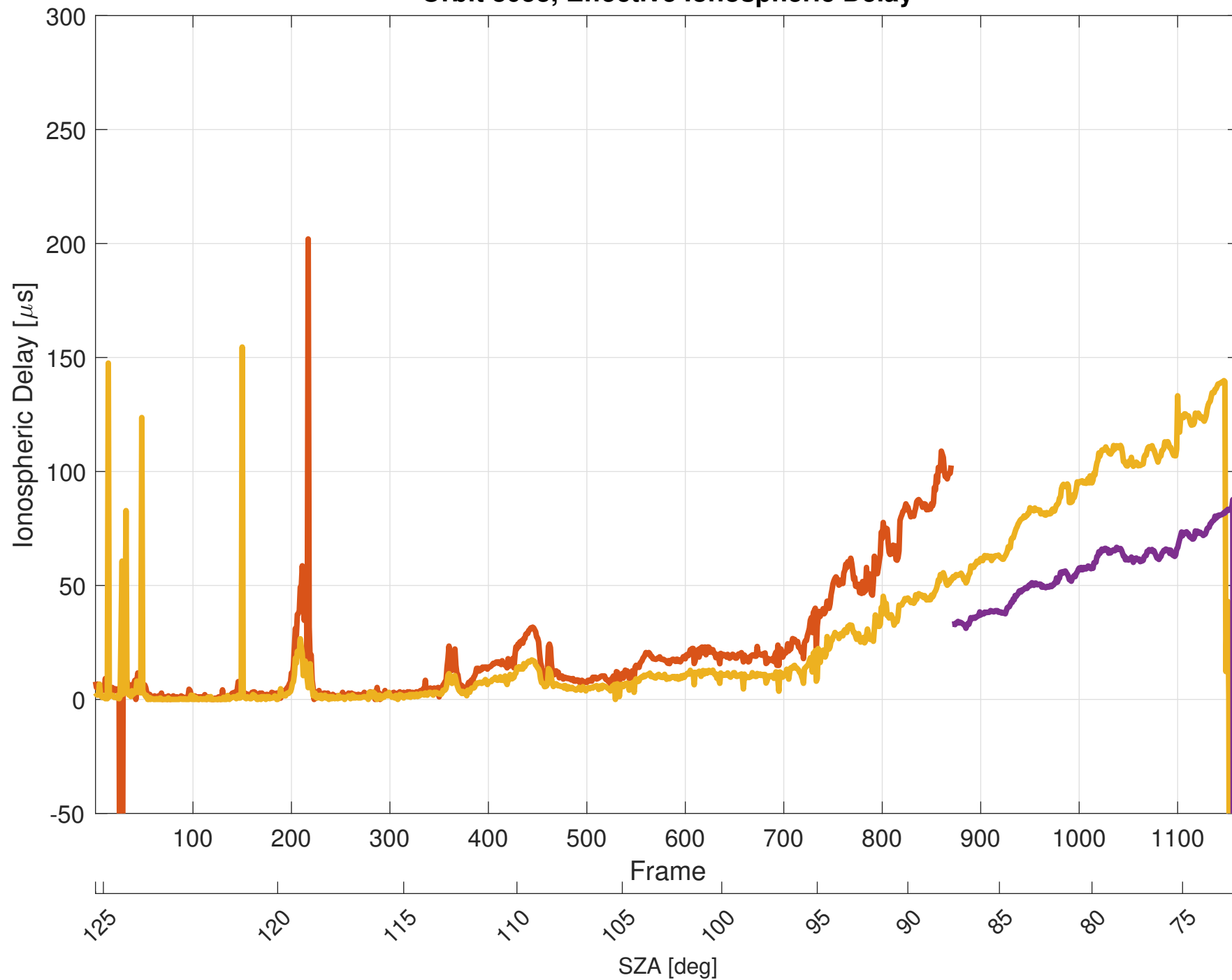
Orbit 8053, Effective Ionospheric Delay
