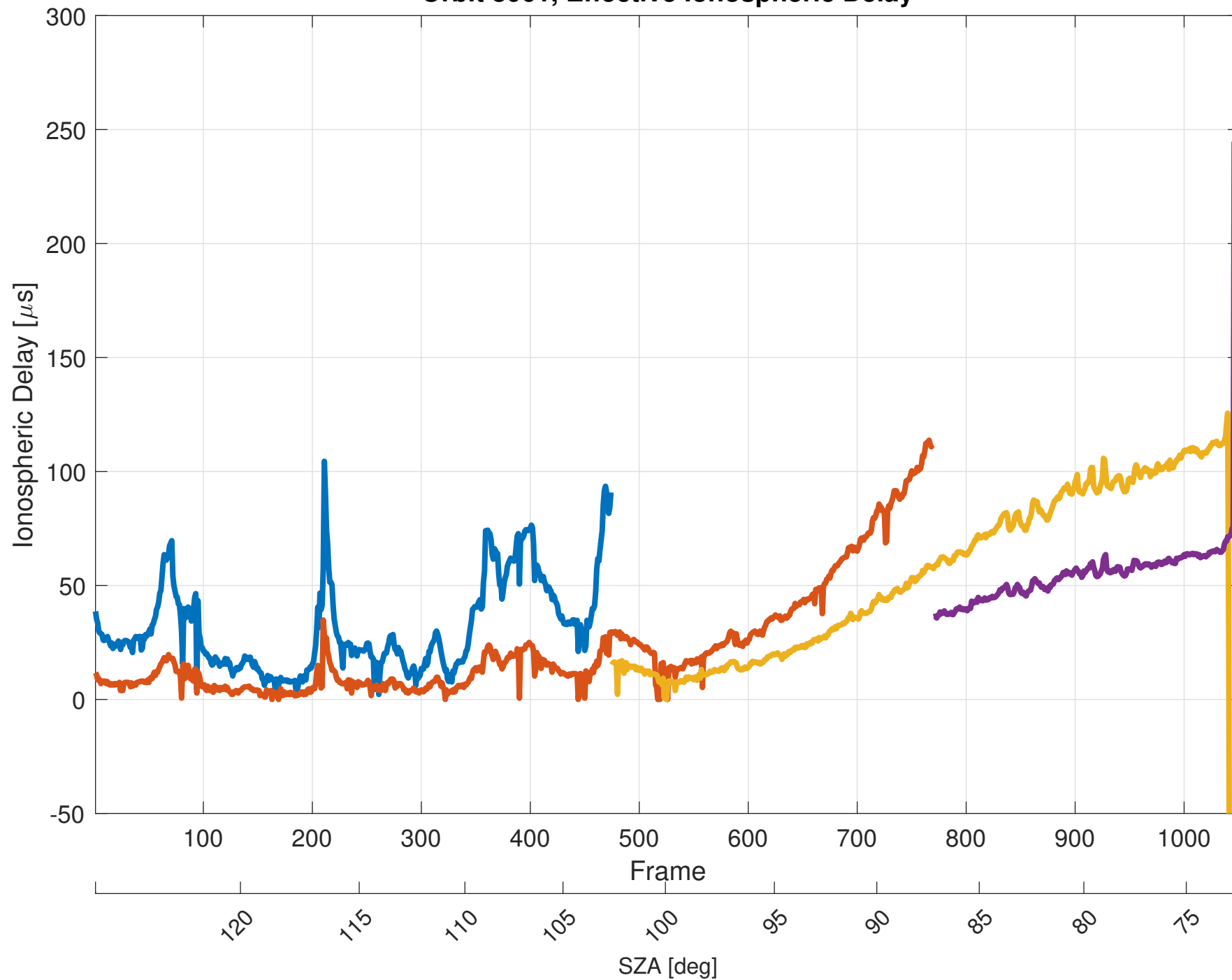
Orbit 8061, Effective Ionospheric Delay
