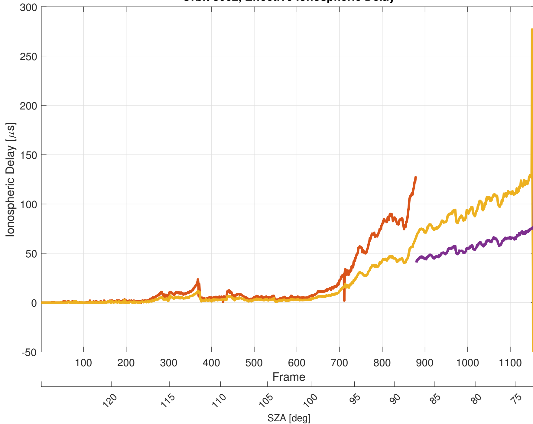
Orbit 8062, Effective Ionospheric Delay
