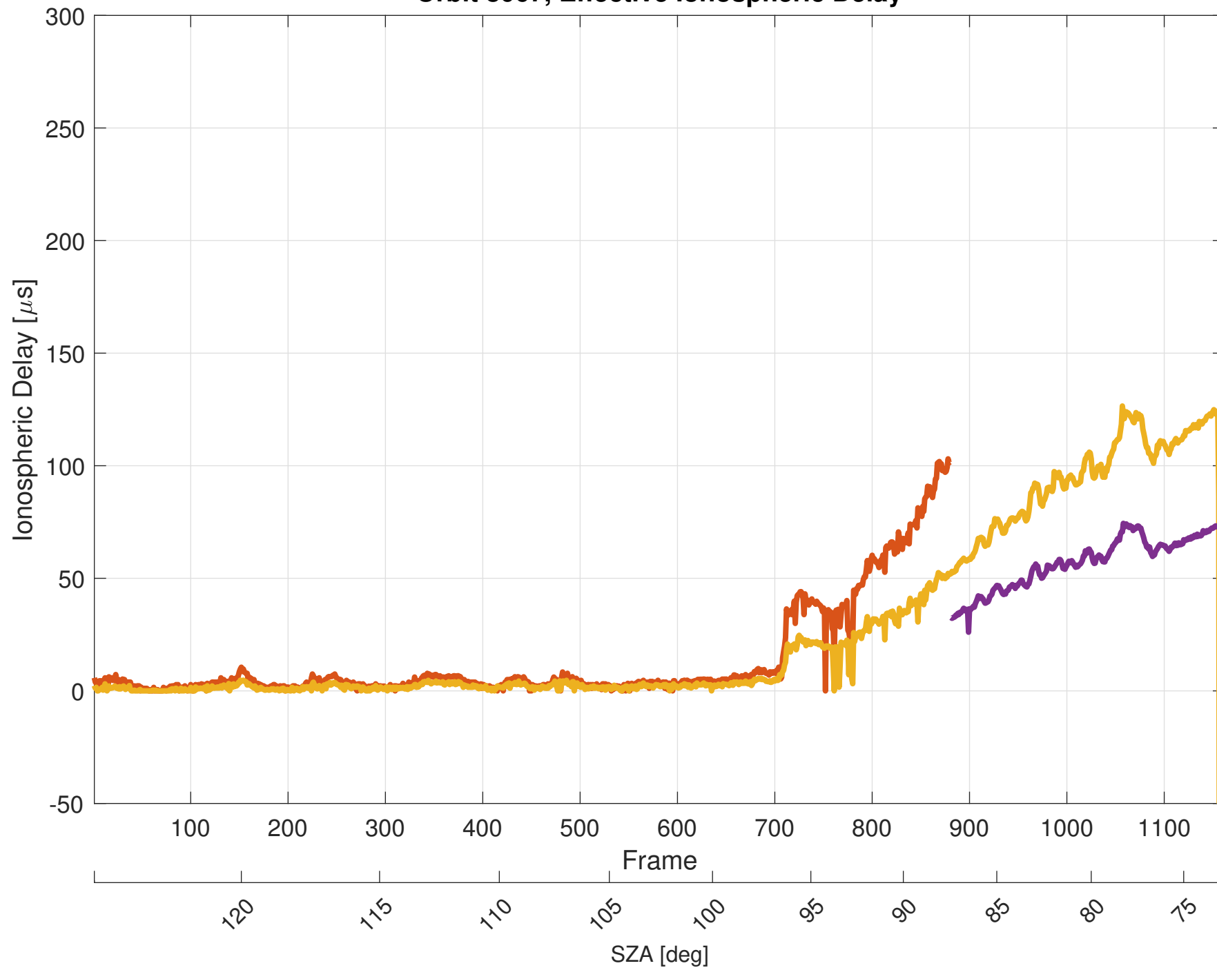
Orbit 8067, Effective Ionospheric Delay
