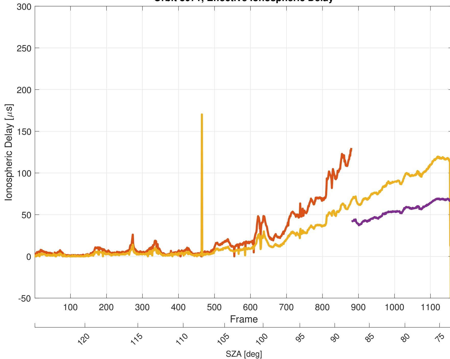
Orbit 8071, Effective Ionospheric Delay
