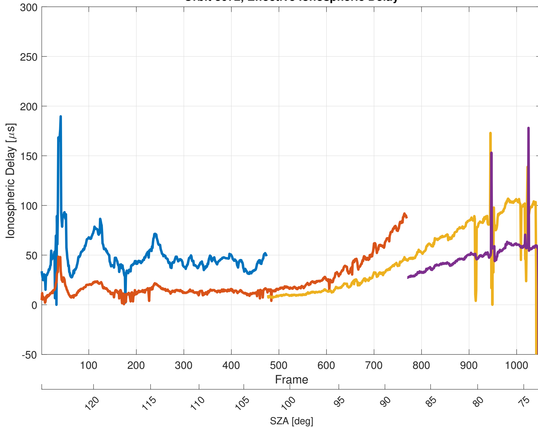
Orbit 8072, Effective Ionospheric Delay
