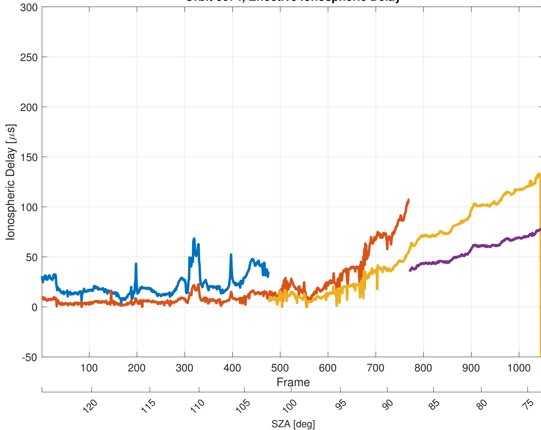
Orbit 8074, Effective Ionospheric Delay
