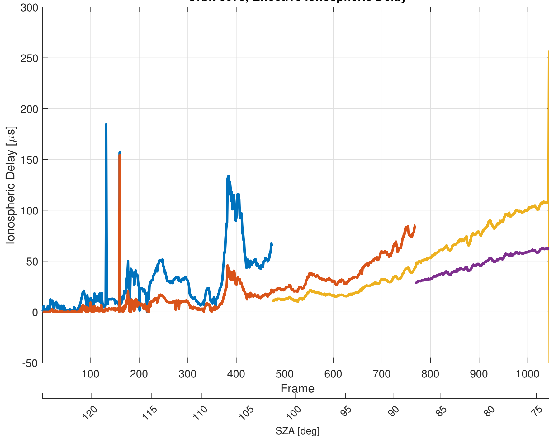
Orbit 8075, Effective Ionospheric Delay
