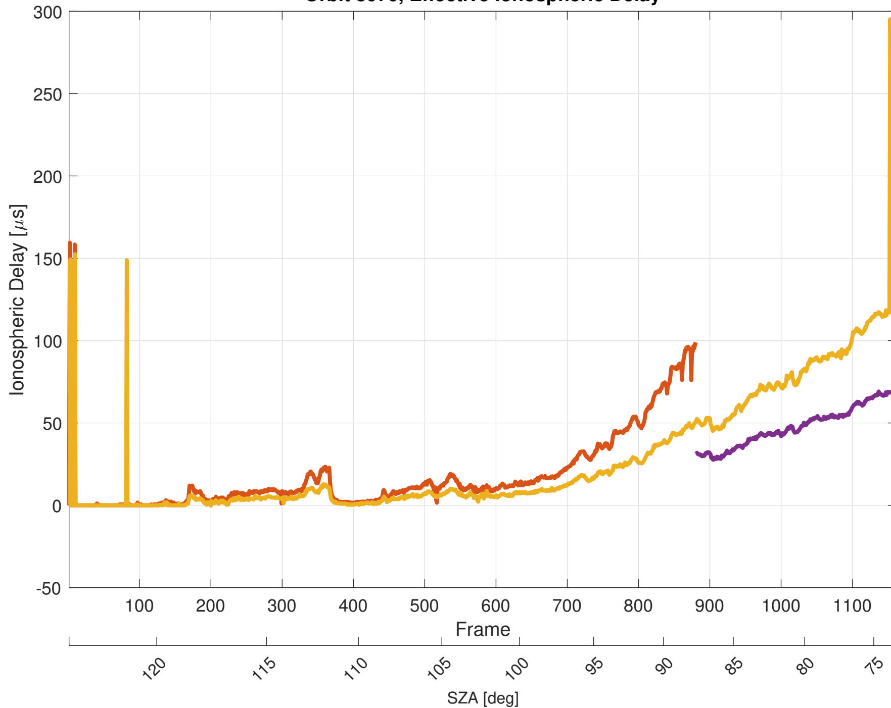
Orbit 8076, Effective Ionospheric Delay
