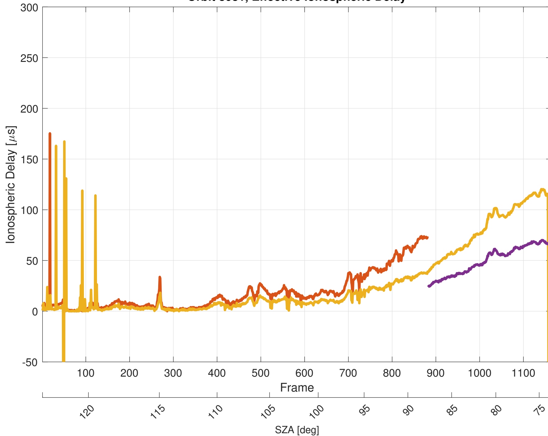
Orbit 8081, Effective Ionospheric Delay
