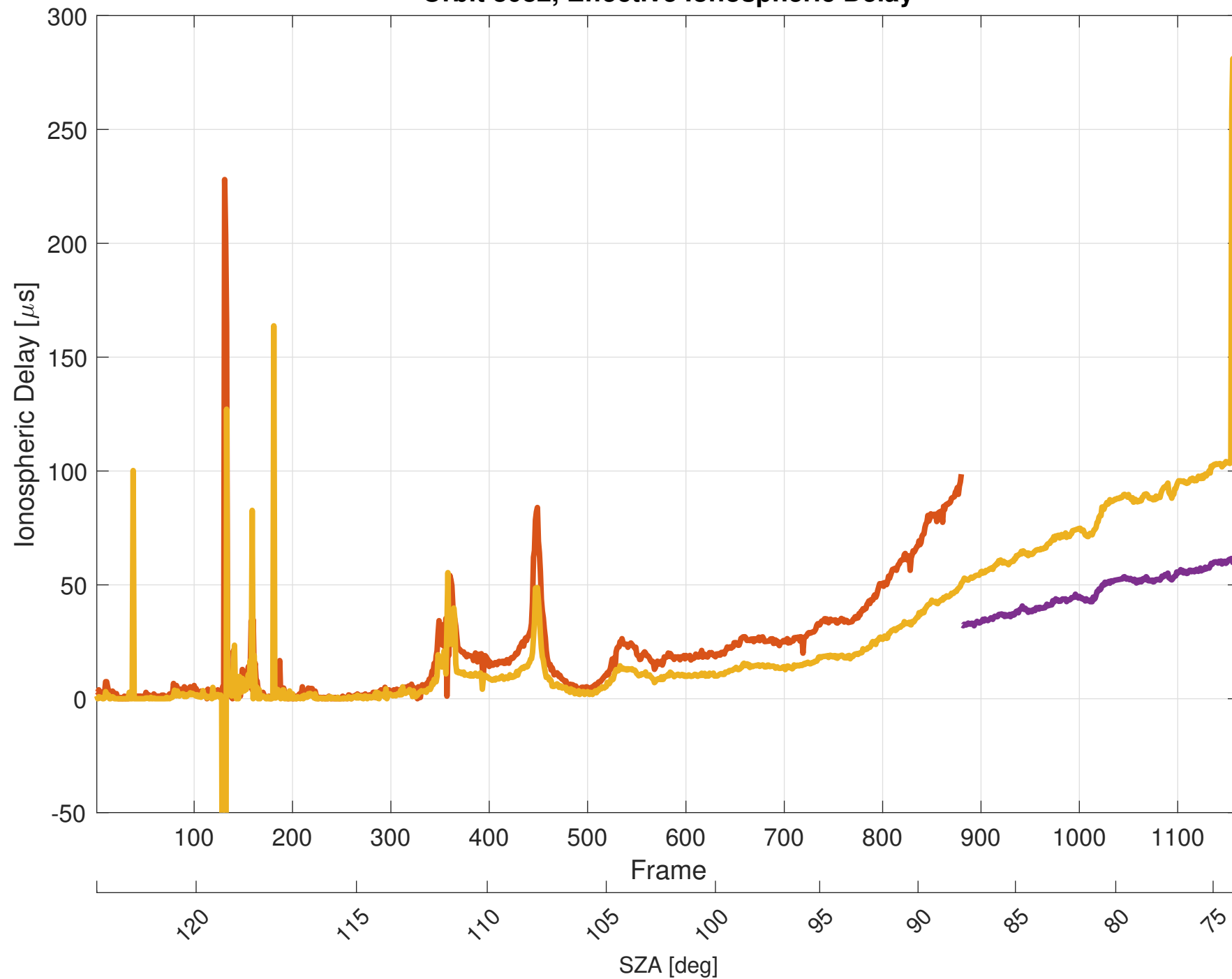
Orbit 8082, Effective Ionospheric Delay
