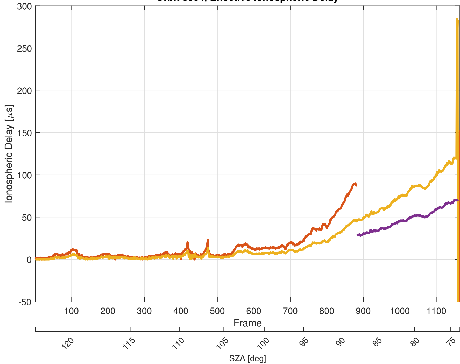
Orbit 8084, Effective Ionospheric Delay
