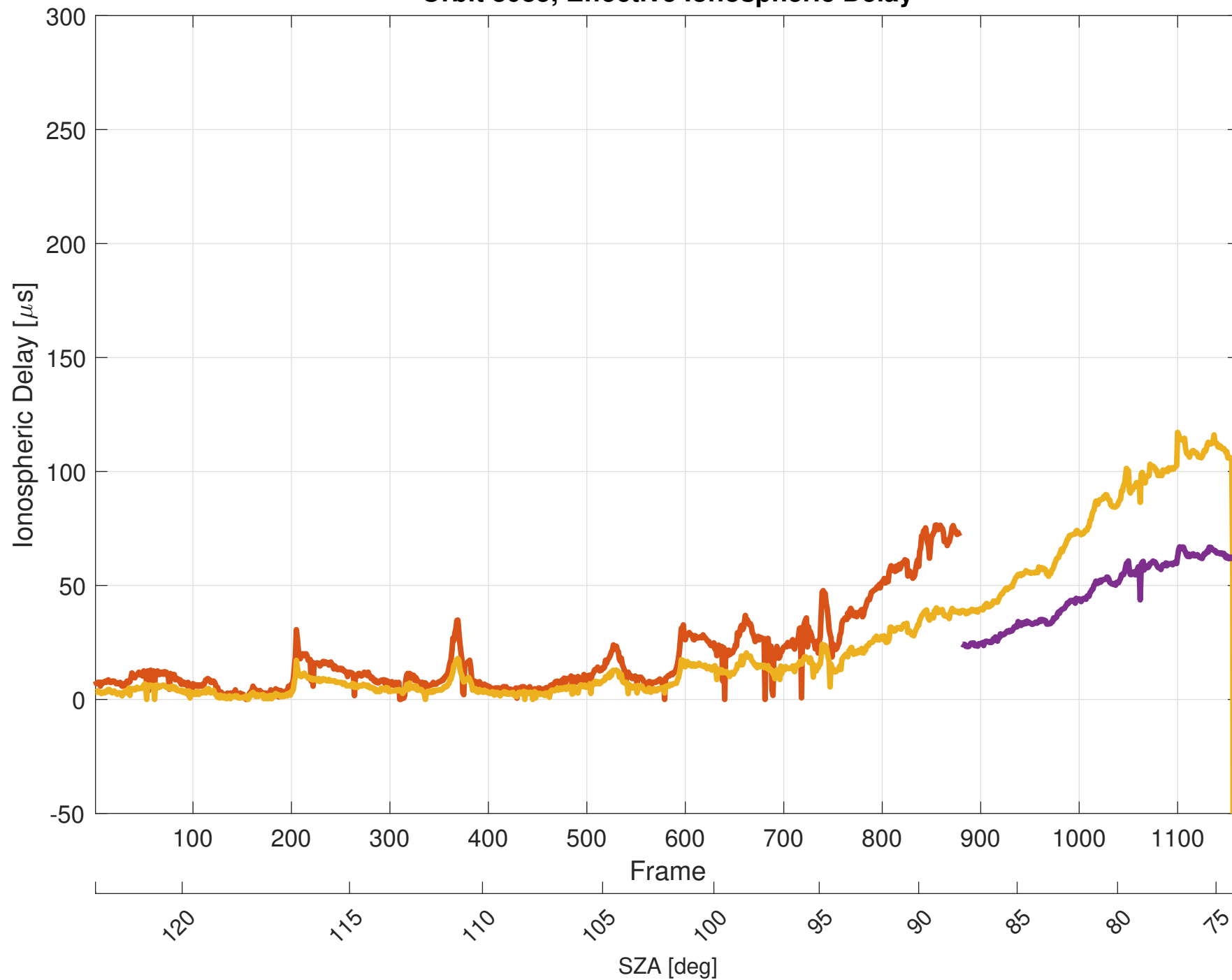
Orbit 8085, Effective Ionospheric Delay
