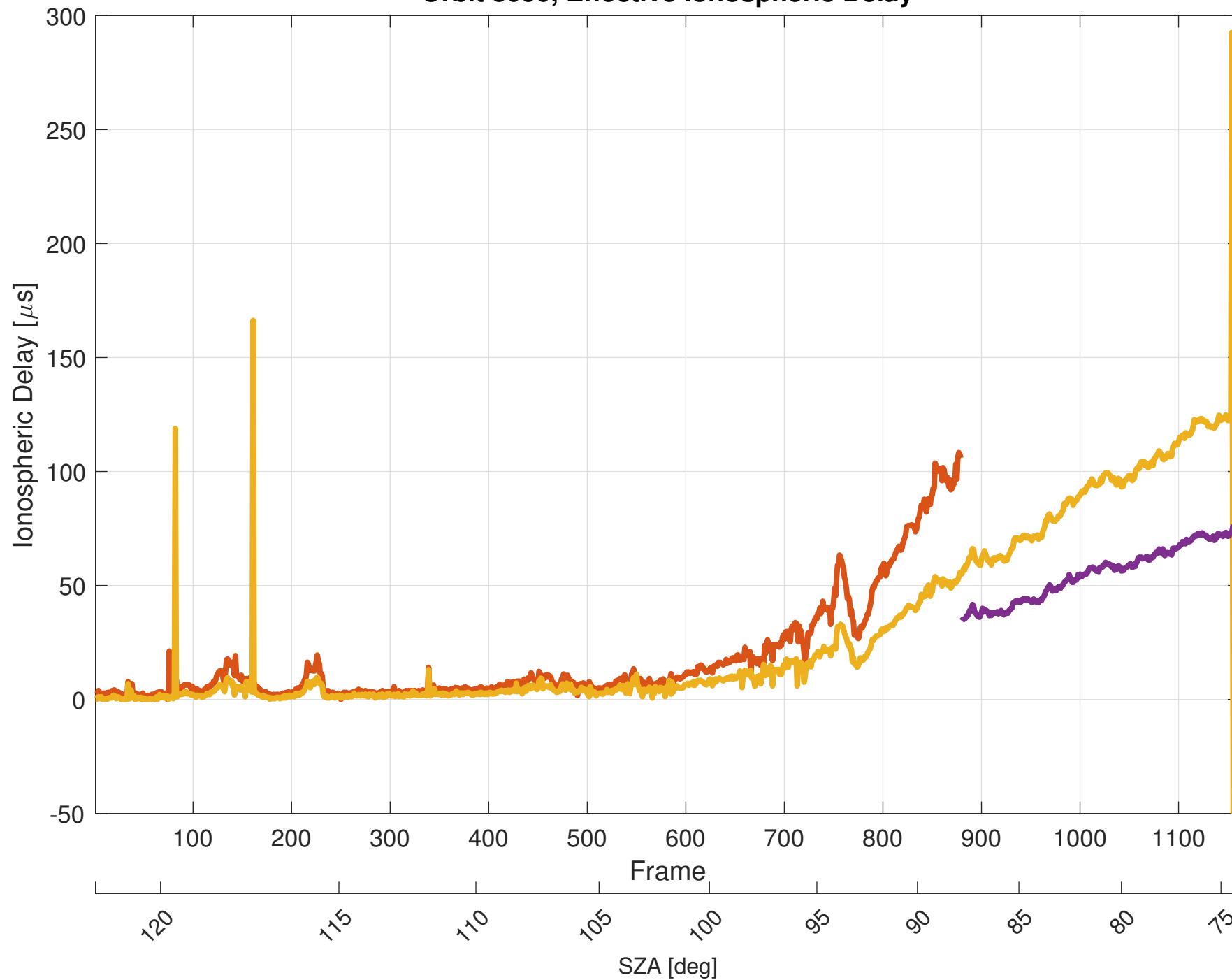
Orbit 8090, Effective Ionospheric Delay
