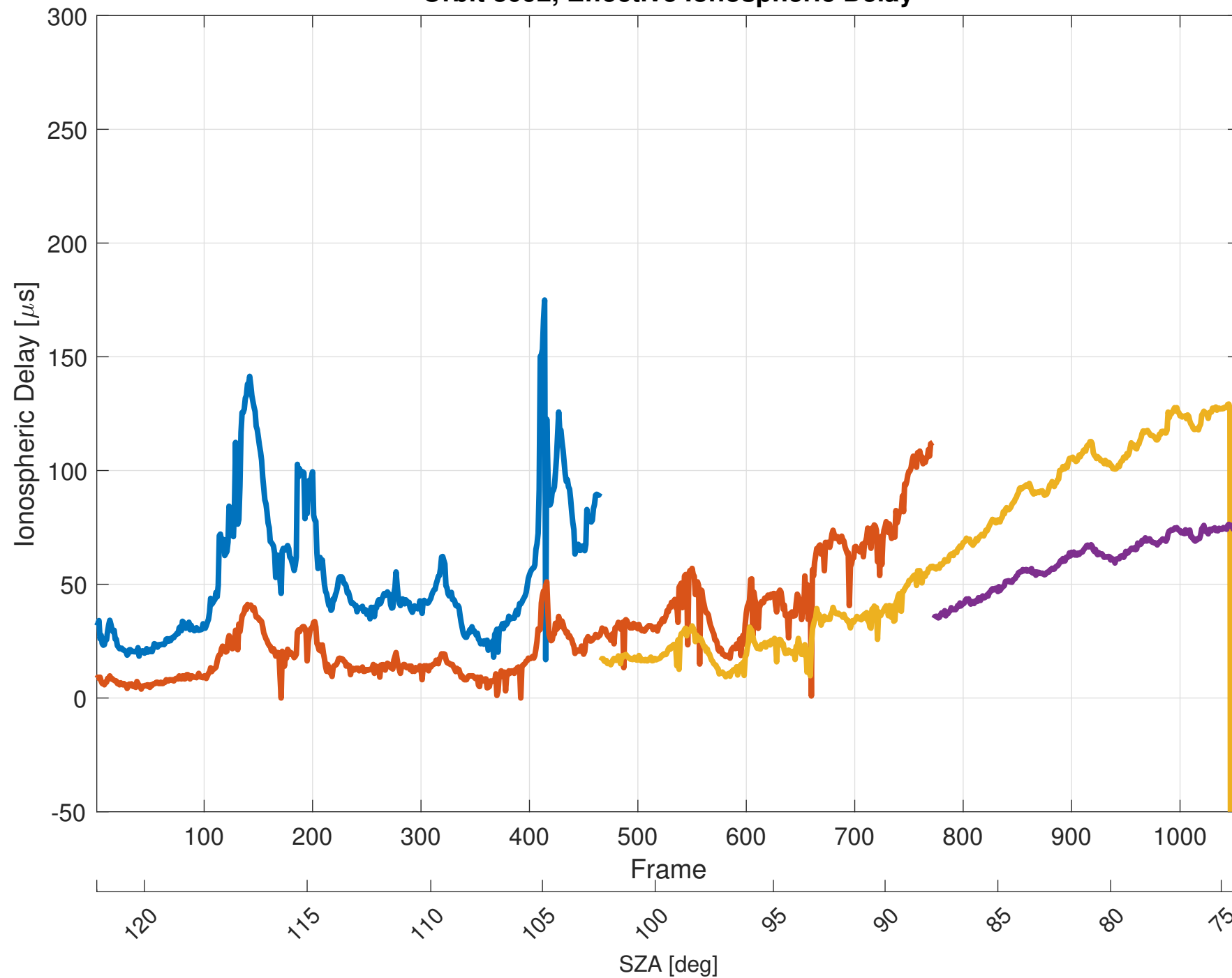
Orbit 8092, Effective Ionospheric Delay
