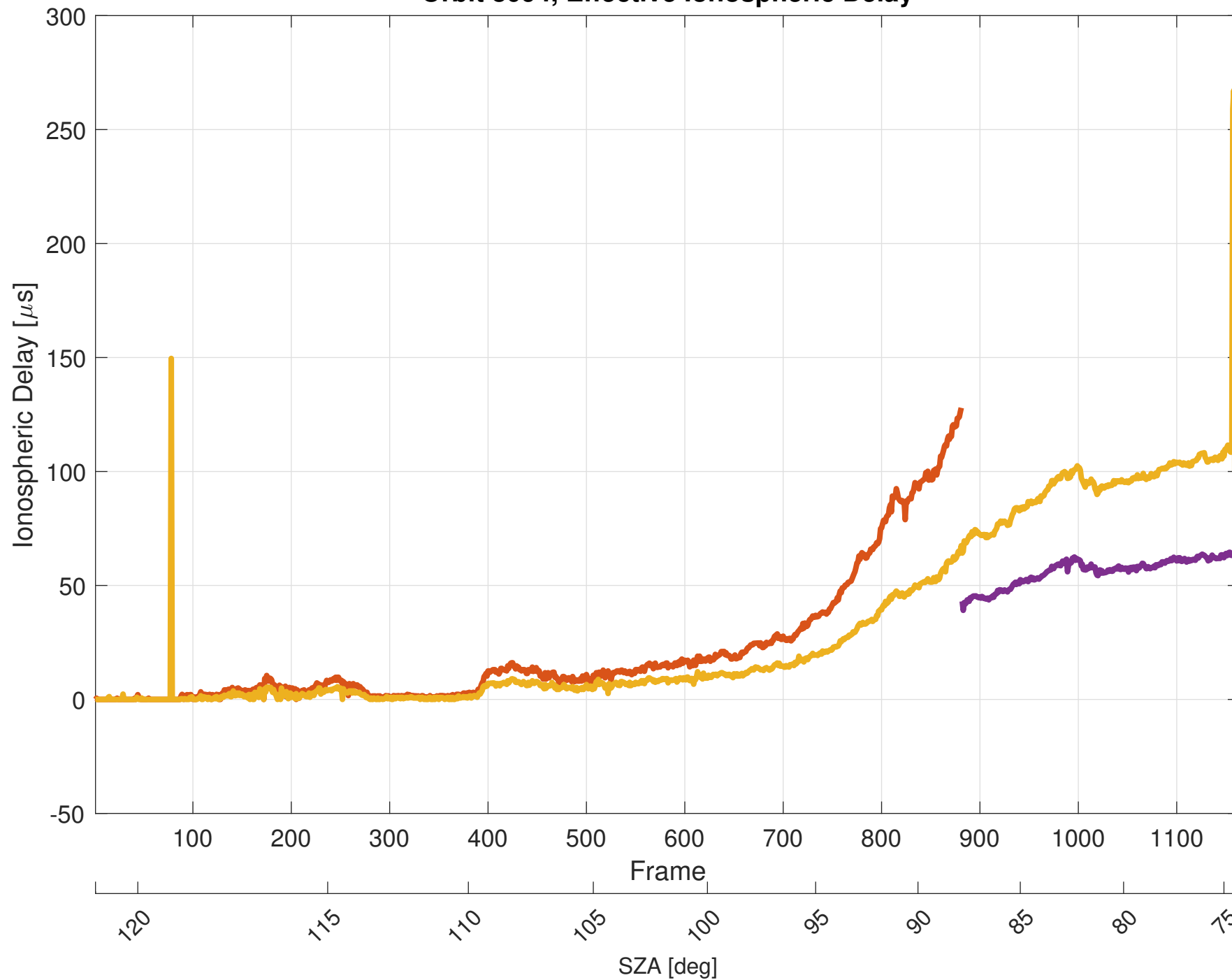
Orbit 8094, Effective Ionospheric Delay
