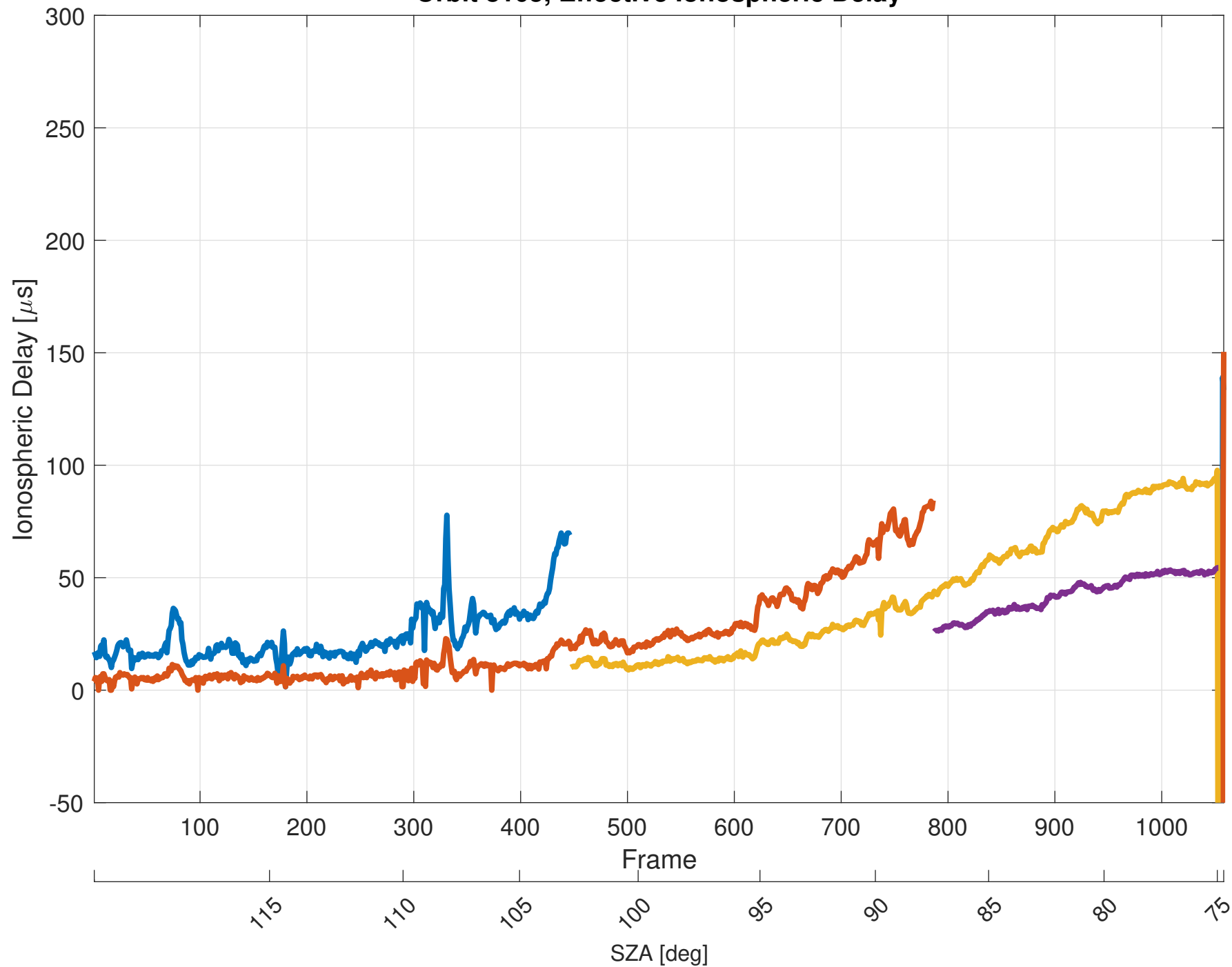
Orbit 8105, Effective Ionospheric Delay
