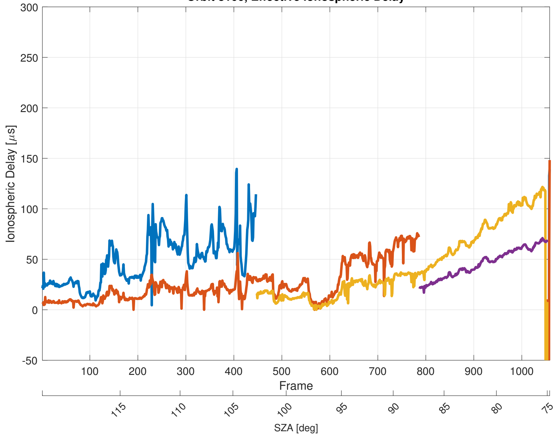
Orbit 8106, Effective Ionospheric Delay
