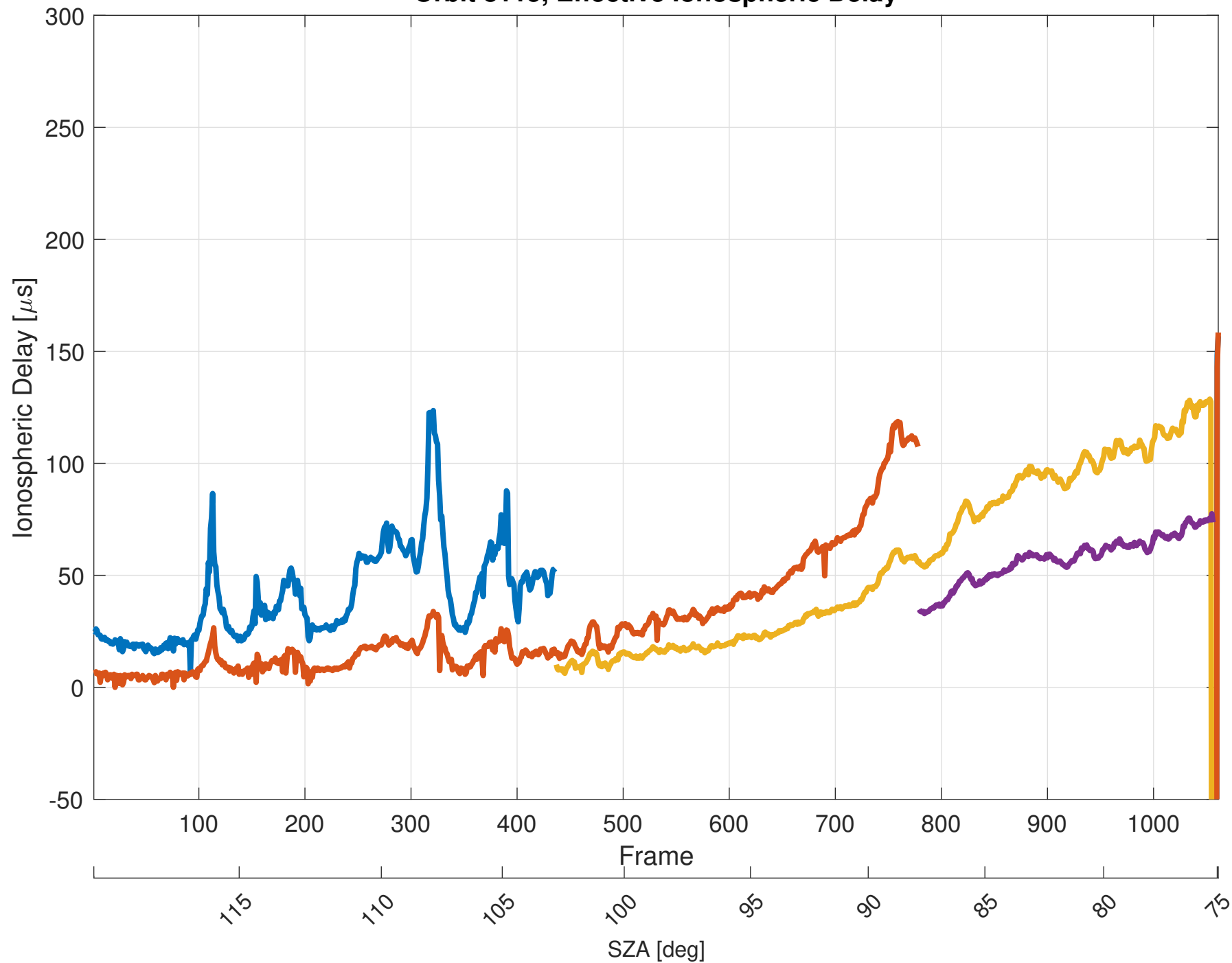
Orbit 8115, Effective Ionospheric Delay
